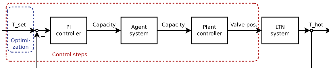
Figure 1: Optimization and control scheme for low temperature networks
