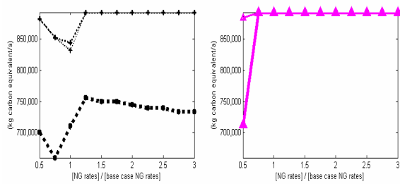
Figure A- 38: Carbon equivalent emissions for volumetric natural gas rate variation and PV subsidies
