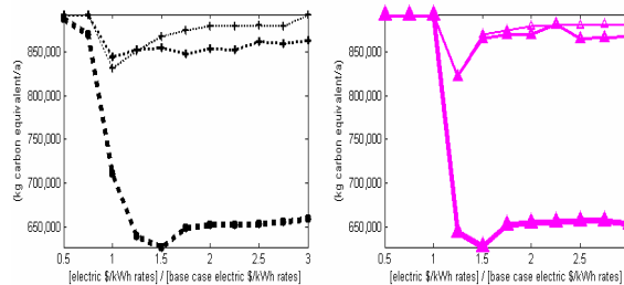
Figure A- 34: Carbon equivalent emissions for volumetric electricity rate variation and PV subsidies
