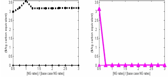
Figure A- 39: Annualized subsidy cost of carbon emissions for volumetric natural gas rate variation and PV subsidies
