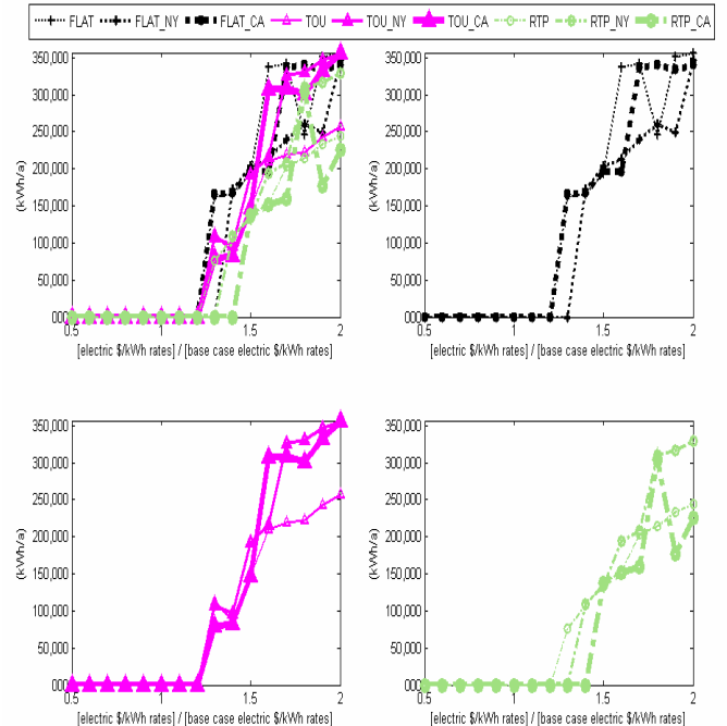
Figure 13: Cooling load offset by recovered heat for volumetric electricity rate sensitivity
