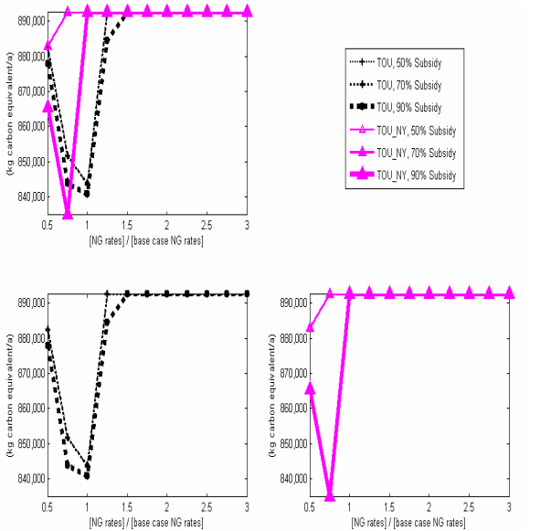
Figure A- 14: Carbon equivalent emissions for volumetric natural gas rate variation and fuel cell subsidies
