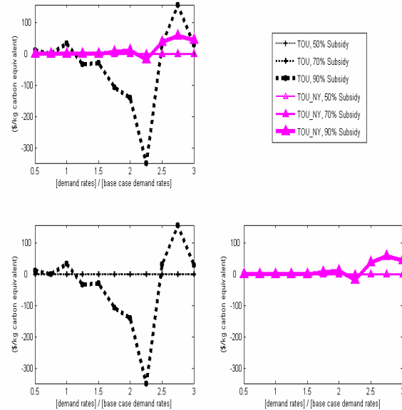
Figure A- 19: Annualized subsidy cost of carbon emissions for as-used demand rate variation and fuel cell subsidies
