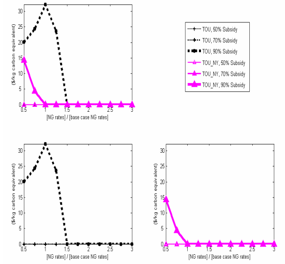
Figure A- 15: Annualized subsidy cost of carbon emissions for volumetric natural gas rate variation and fuel cell subsidies
