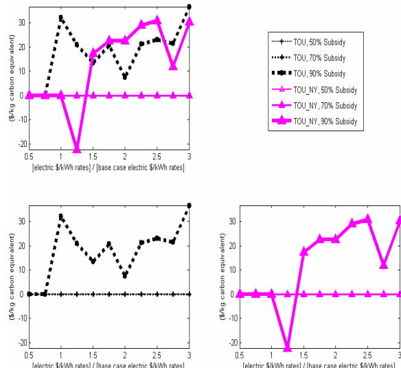
Figure A- 11: Annualized subsidy cost of carbon equivalent savings for volumetric electricity rate variation and fuel cell subsidies
