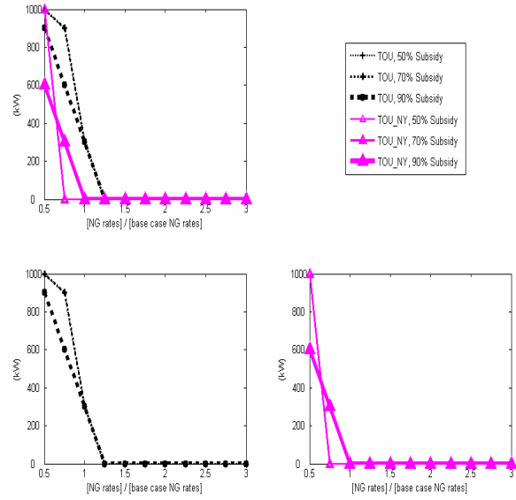
Figure A- 13: Installed electrical capacity of natural gas engines for volumetric natural gas rate variation and fuel cell subsidies
