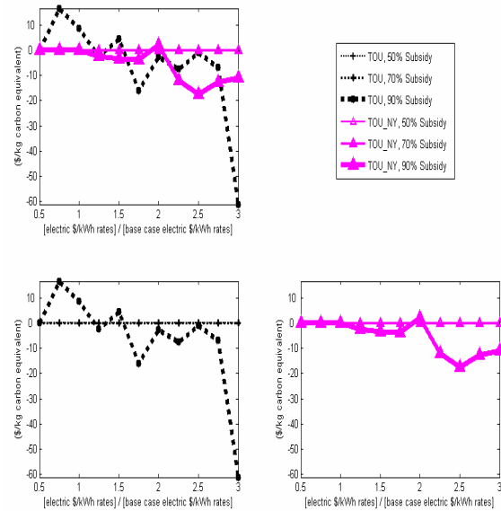
Figure A- 23: Annualized subsidy cost of carbon equivalent savings for volumetric electricity rate variation and microturbine subsidies
