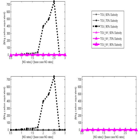
Figure A- 27: Annualized subsidy cost of carbon emissions for volumetric natural gas rate variation and microturbine subsidies
