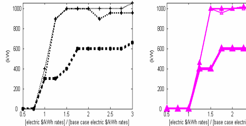
Figure A- 33: Installed electrical capacity of natural gas engines for volumetric electricity rate variation and PV subsidies
