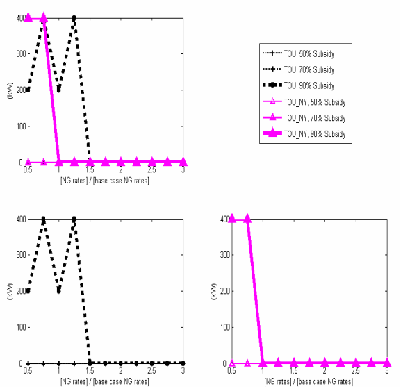
Figure A- 12: Installed electrical capacity of fuel cells for volumetric natural gas rate variation and fuel cell subsidies
