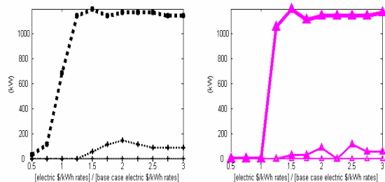
Figure A- 32: Installed electrical capacity of PV for volumetric electricity rate variation and PV subsidies
