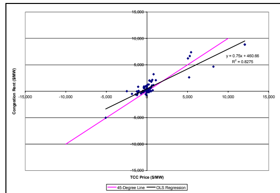
Figure 57. TCC Price Paid and Congestion Rent Collected (100% Data for Round 5 Autumn 2001 Unique Award Auction)
