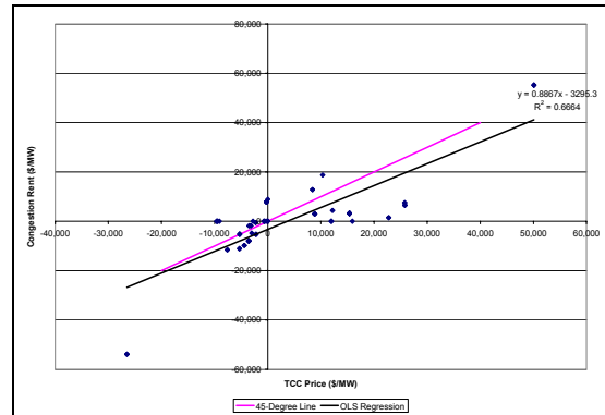
Figure 10. TCC Price Paid and Congestion Rent Collected (90% Data for Round 3 Spring 2000 Total Award Auction)
