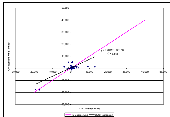
Figure 22. TCC Price Paid and Congestion Rent Collected (90% Data for Round 3 Spring 2001 Total Award Auction)
