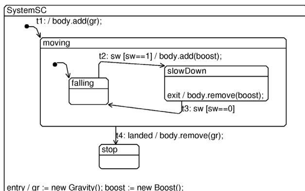
Figure 1: Statechart of a landing device
