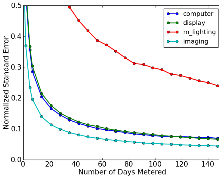
Figure 6. Normalized standard error for different metering periods, shown for computers, displays, plugged lighting, and imaging equipment
