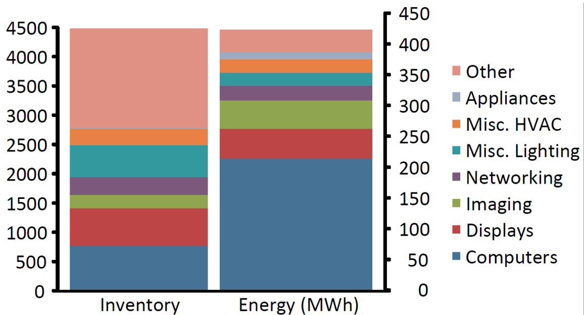
Figure 2. Inventory and Estimated Annual Energy Consumption, for the Top 7 Energy-Consuming Device Categories
