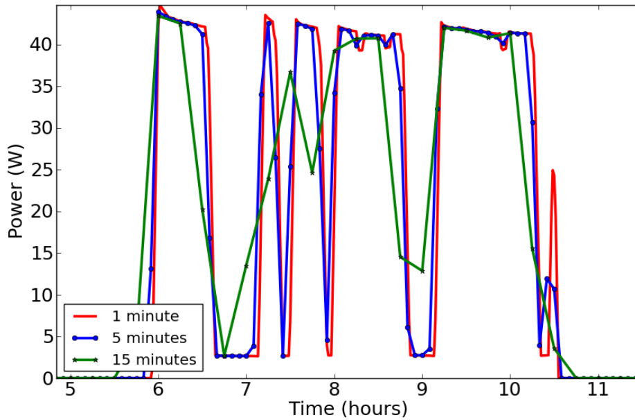
Figure 7. Time series data of a LCD computer display shown for three different data sampling rates.
