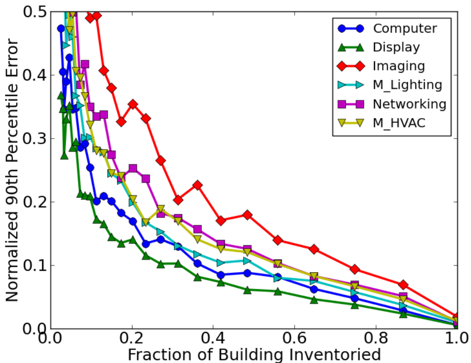
Figure 5 Normalized 90th Percentile Error vs. Fraction of Building Inventoried
