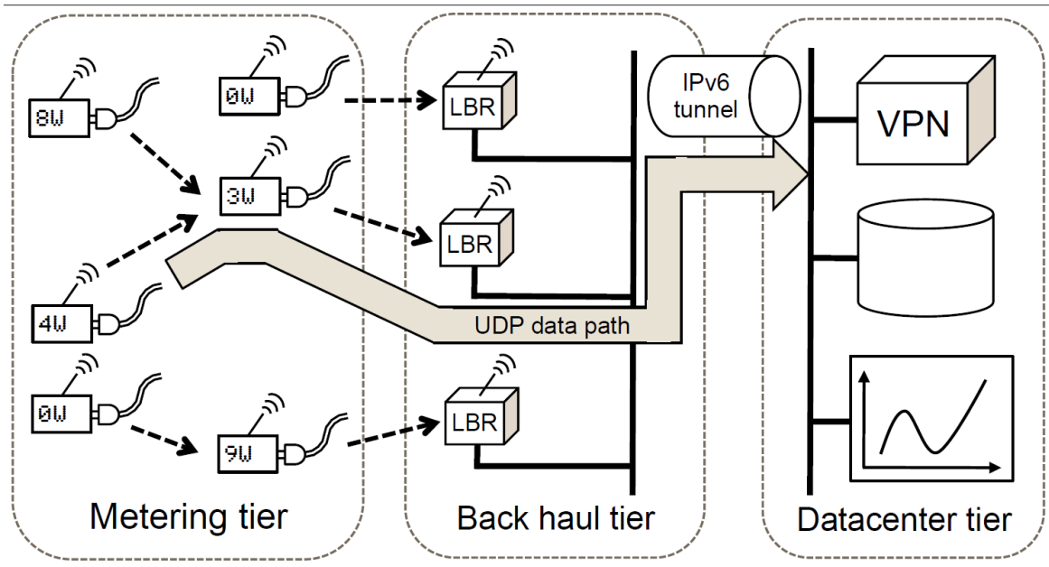
Figure 4. ACme system network design
