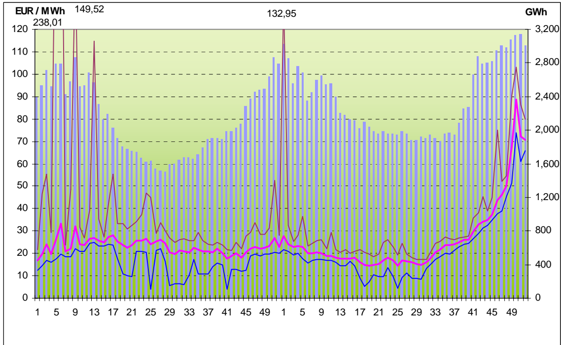
Figure B-3: ELSpot Prices & Volume CY01-02 [ http://www.nordpoolspot.com/ ]
