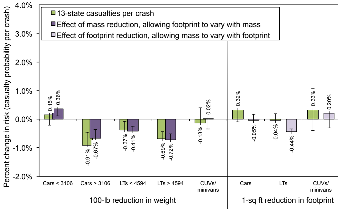
Figure 3.3. Effect of reduction in mass or footprint on 13-state casualty risk per crash, by vehicle type: holding footprint constant, allowing footprint to vary with mass, and allowing mass to vary with footprint
