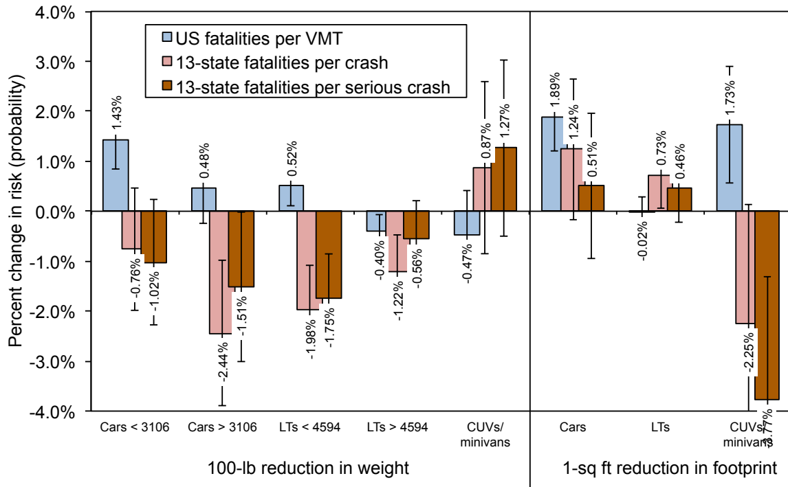
Figure 2.10. Effect of mass and footprint reduction on three types of risk, by vehicle type
