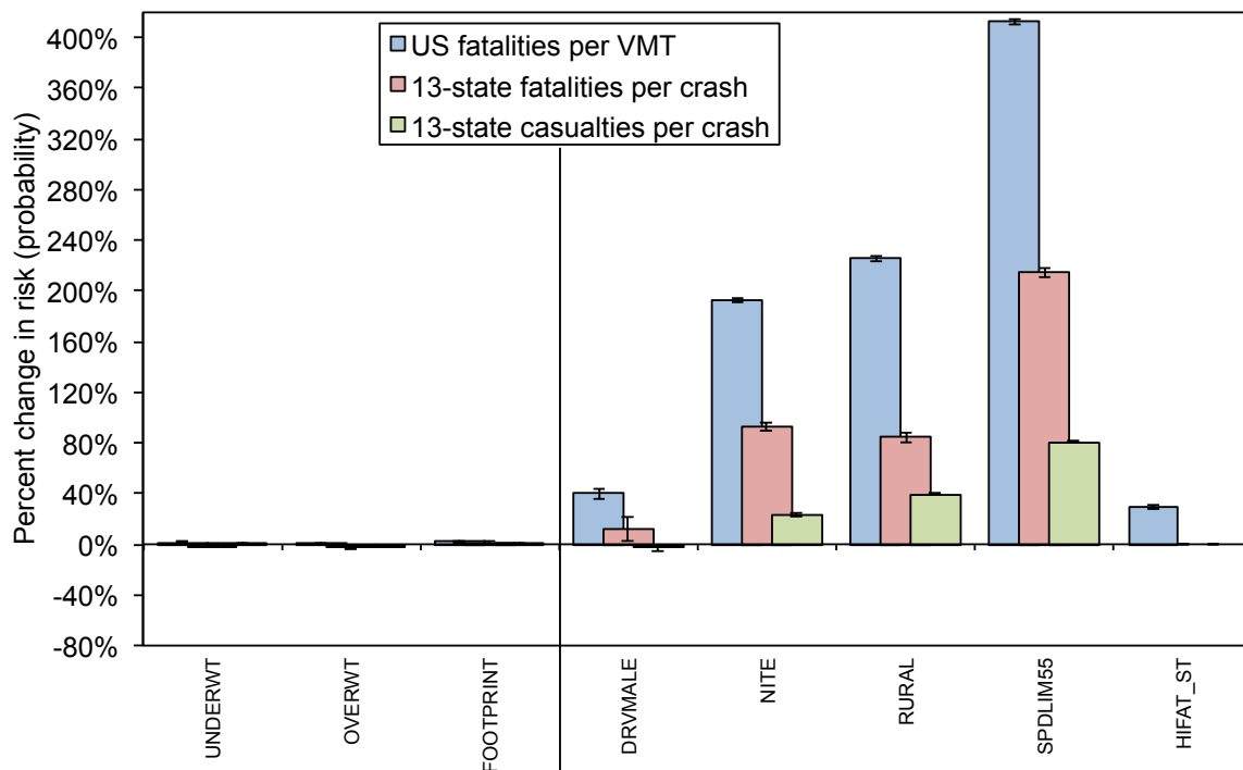
Figure 2.16. Effect of mass and footprint reduction, and selected control variables, on 13-state casualty risk per crash, passenger cars
