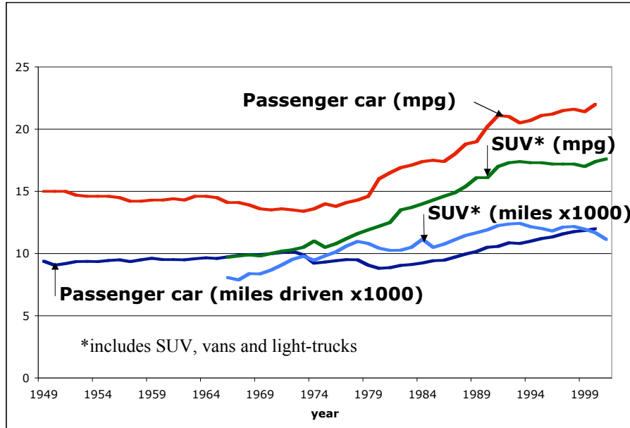
Figure 6. Passenger & SUV Fuel Efficiency and Vehicle Mileage 1949-2000
