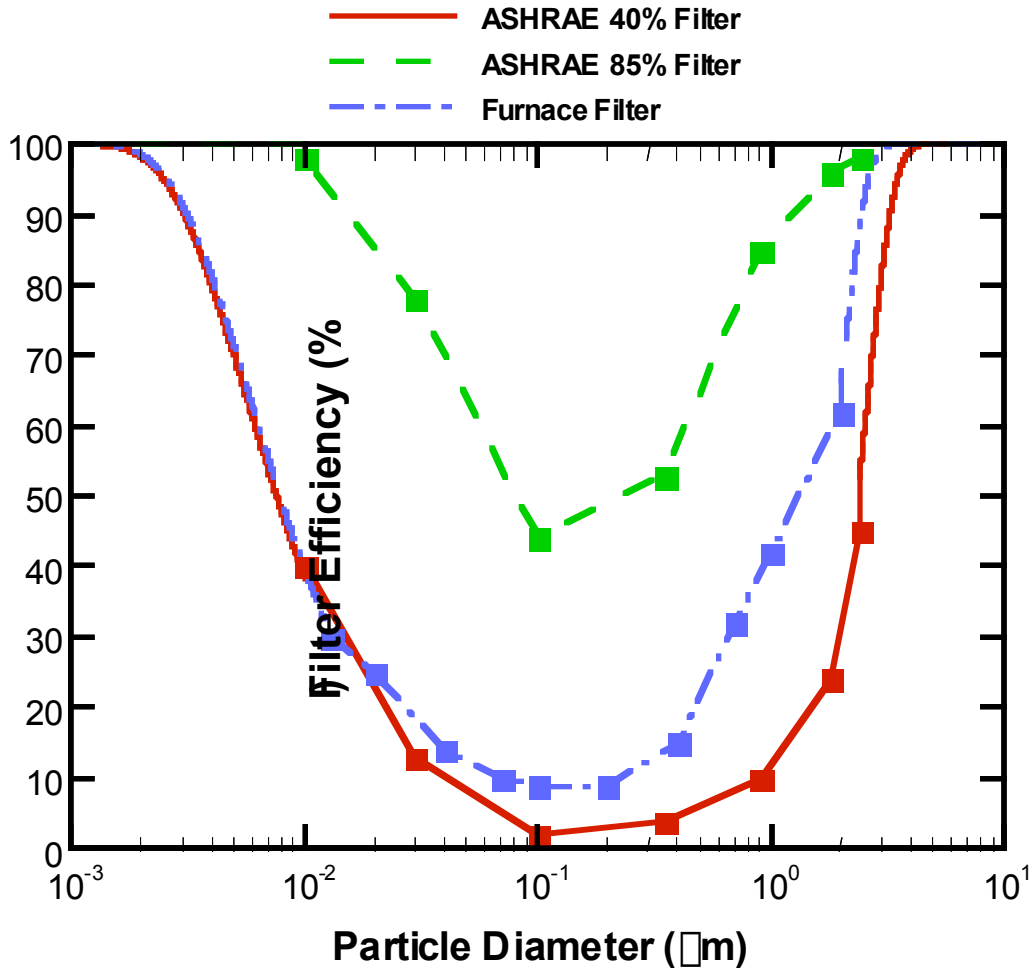
Figure 3.3.1 Filter efficiency data from Hanley et al. (1994) along with best fit lines from Riley et al. (2001).
