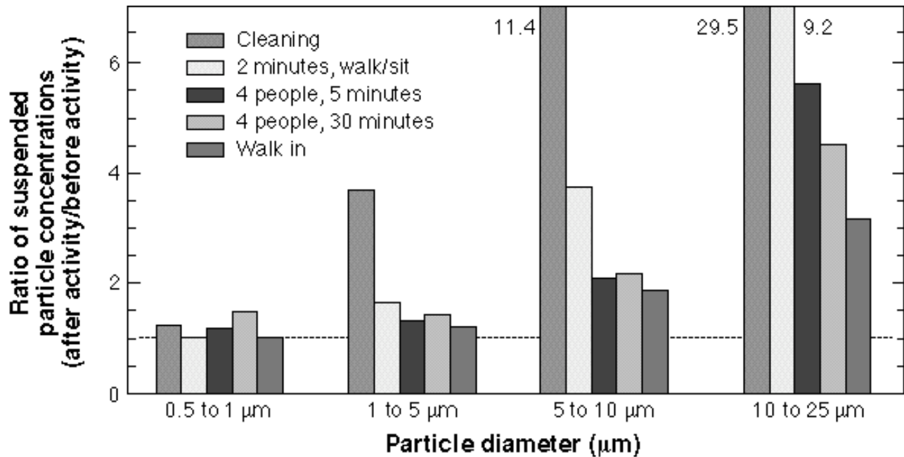
Figure 3.4 Ratios of suspended particle concentrations after human activities to concentrations before activity in a single-family residence (from Thatcher and Layton (1995) ).
