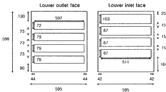
Fig.2. Opening Areas of the Louver with Dimensions in mm
