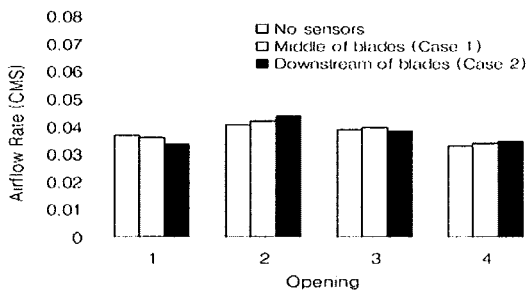
Fig.12. Relative Airflow Rates through Openings (0.15 m 3 /s)
