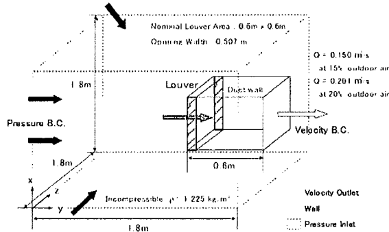
Fig.1. CFD Calculation Domain
