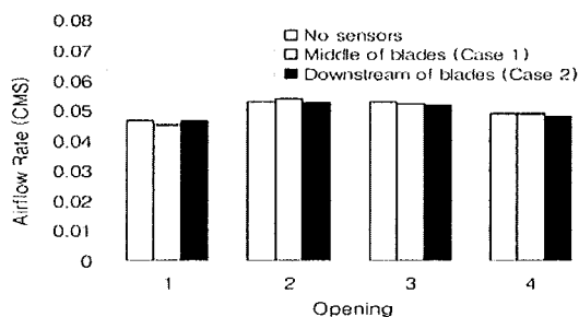
Fig.13. Relative Airflow Rates through Openings (0.20 m 3 /s)
