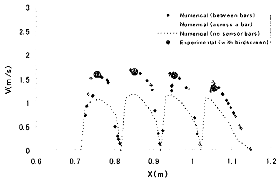
Fig.8. Velocity Magnitude between Blades with Sensors Mounted for Case 1 ( Q=0.15 \text{ m}^3/\text{s} )
