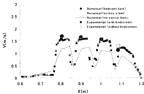
Fig.9. Velocity Magnitude Downstream of Blades with Sensors Mounted for Case 2 ( Q=0.15 \text{ m}^3/\text{s} )
