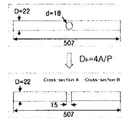
Fig.4. Geometry of a Velocity Probe with Actual Opening for a Velocity Sensor (Top) and with Simplified Geometry Used in Modeling with Dimensions in mm
