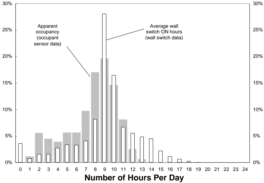
Figure 10. Average lighting ON hours per day (calculated from the wall switch data) for 14 5th floor offices for occupied days between June 1 and December 31, 1998. Apparent occupancy (occupant sensor data) for the same data set is shown with gray bars. The apparent occupancy includes the occupant sensor time delays and
