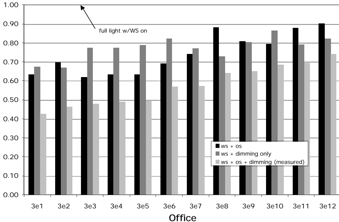
Figure 14. Task Tuning: Average normalized lighting energy use for 12 private offices using task tuning for occupied weekdays for the period June-December 1998 (3rd floor East). 2nd column reflects room geometry.
