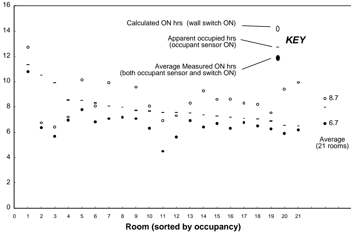
Figure 4. Average hours per day that lighting is ON as measured using occupant sensor control and as calculated based on wall switch use only for 21 offices on the 3rd floor. Data are for occupied weekdays from June
