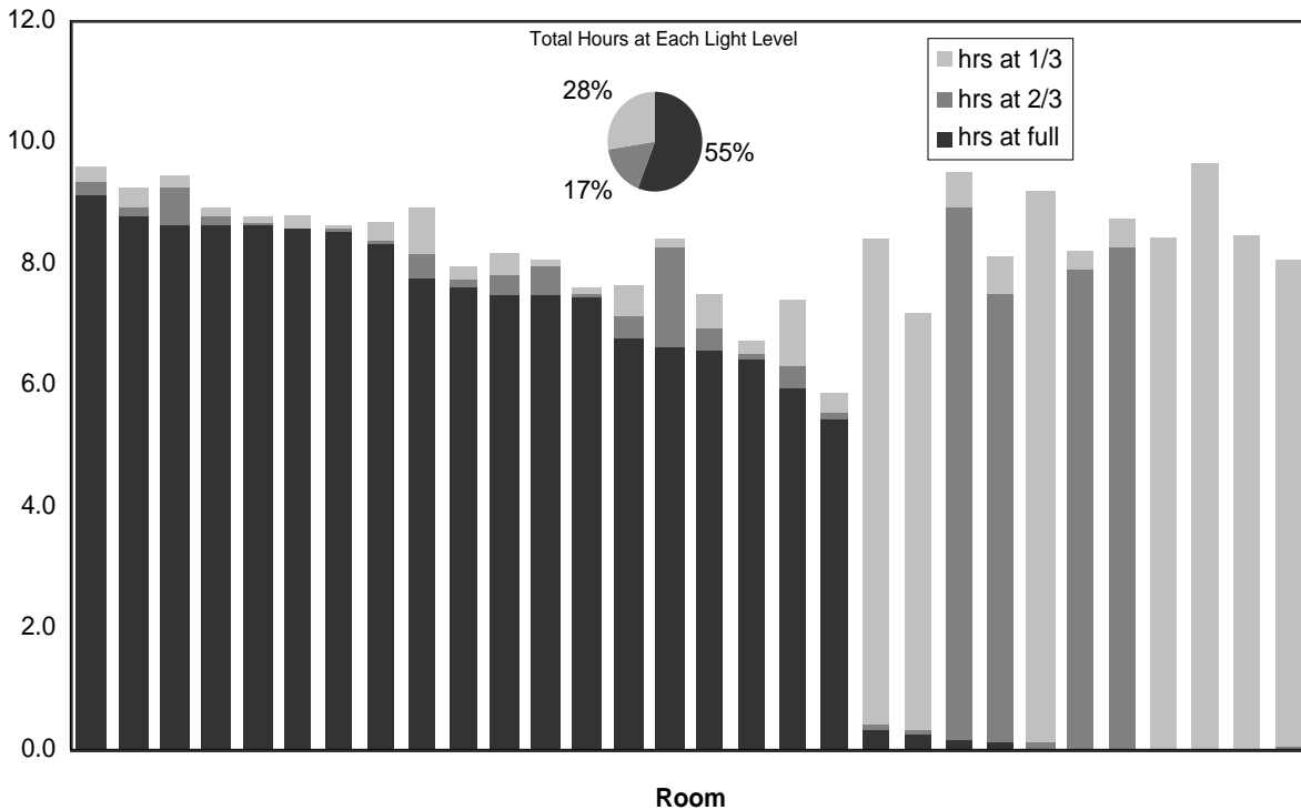
Figure 12. Average hours per day at 1/3, 2/3 or full light levels for 30 private daylit offices on the 4th floor. Data are for 2527 occupied office-days between June 1 and December 31, 1998, sorted by full-light hours.
