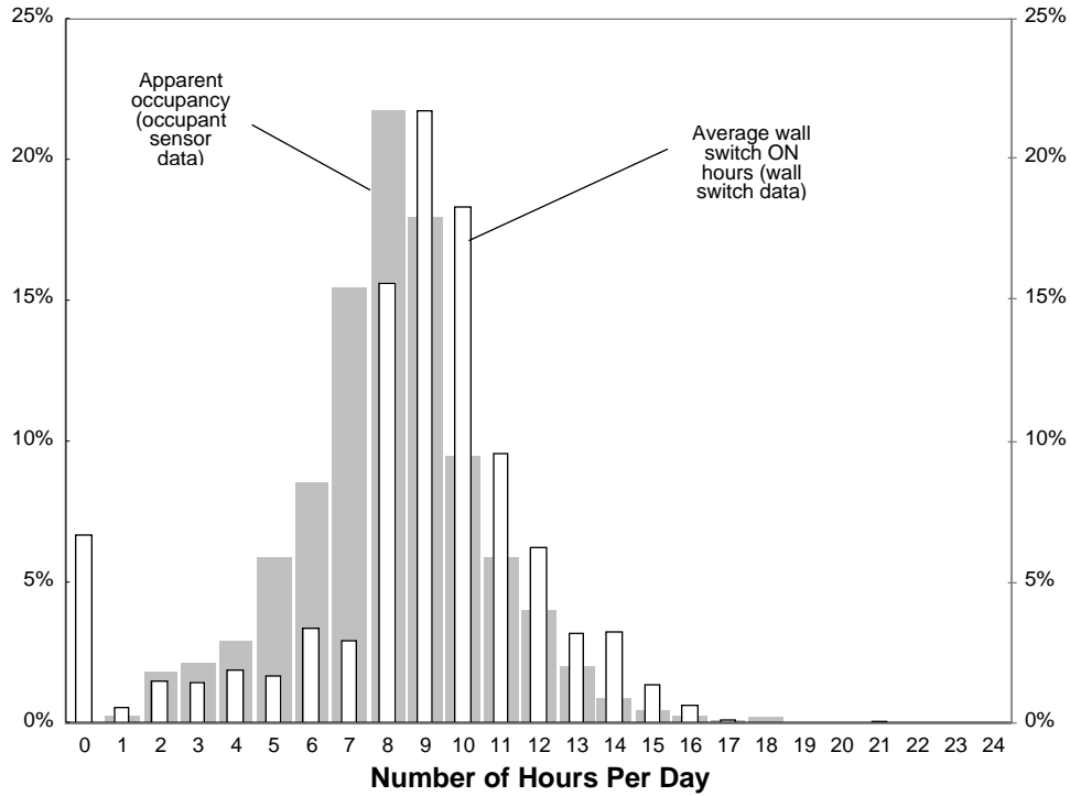
Figure 8. Average lighting ON hours per day (calculated from the wall switch data) for 21 offices on the 3rd floor for occupied days between June 1 and December 31, 1998. Apparent occupancy (occupant sensor data) for the same data set is shown with gray bars. The apparent occupancy includes the occupant sensor time
