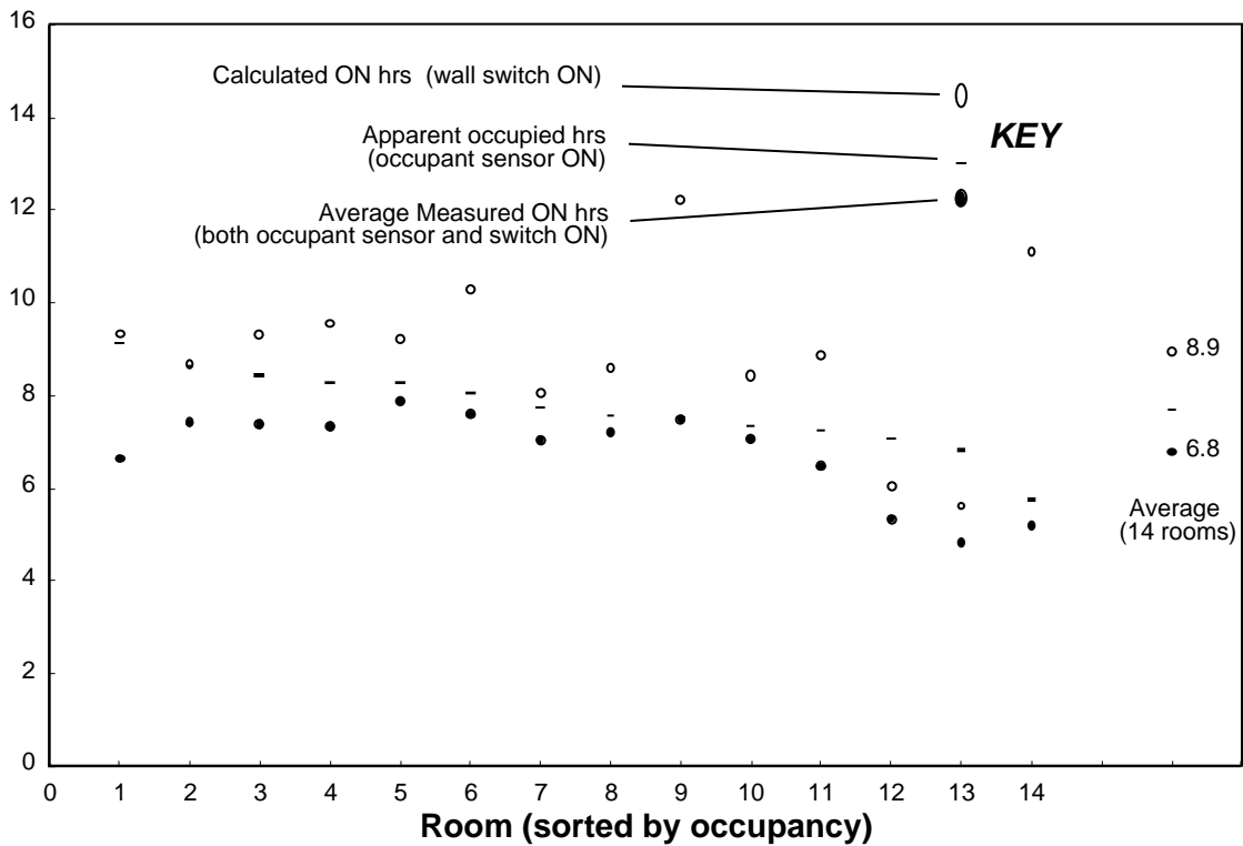
Figure 5. Average hours per day that lighting is ON as measured using occupant sensor control and as calculated based on wall switch use only for 14 offices on the 5th floor. Data are for occupied weekdays from June 1 to December 31, 1998.
