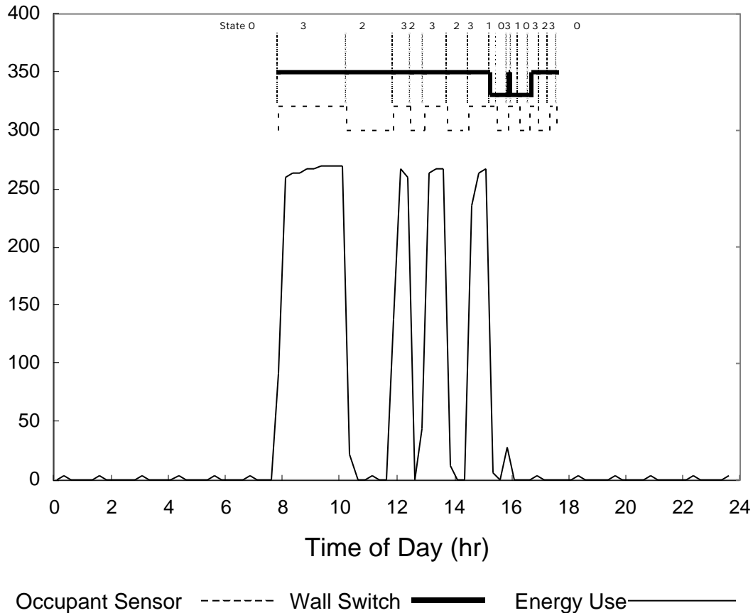
Figure 2. Lighting power, wall switch operation and occupant sensor operation as a function of time of day for a typical private office on the 3rd floor. The resultant lighting use states are marked above the graph.
