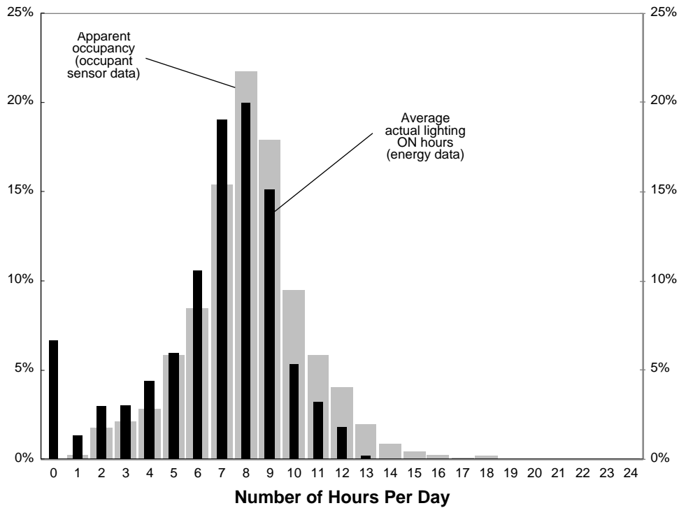
Figure 9. Average lighting ON hours per day for the 21 3rd floor offices (both light switch and occupant sensor ON) for occupied days between June 1 and December 31, 1998. Apparent occupancy (occupant sensor data) for the same data set is shown with gray bars. The apparent occupancy includes the occupant sensor time
