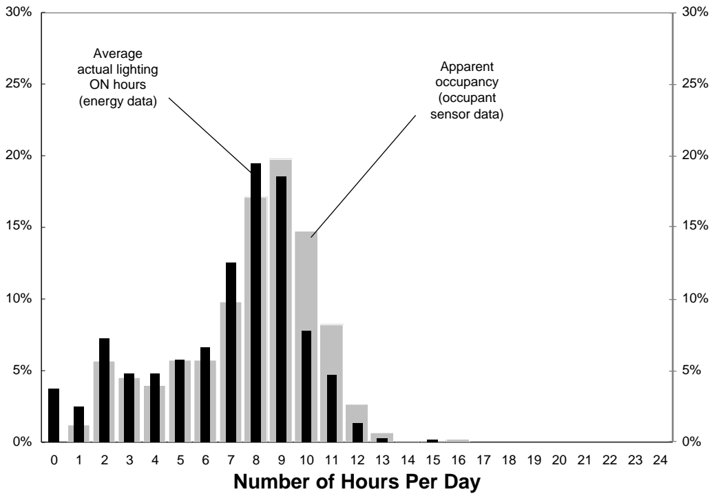
Figure 11. Average lighting ON hours per day for the 14 5th floor offices (both occupant sensor and switch ON) for occupied days between June 1 and December 31, 1998. Apparent occupancy (occupant sensor data) for the same data set is shown with gray bars. The apparent occupancy includes the occupant sensor time delays and therefore overestimates actual occupancy.
