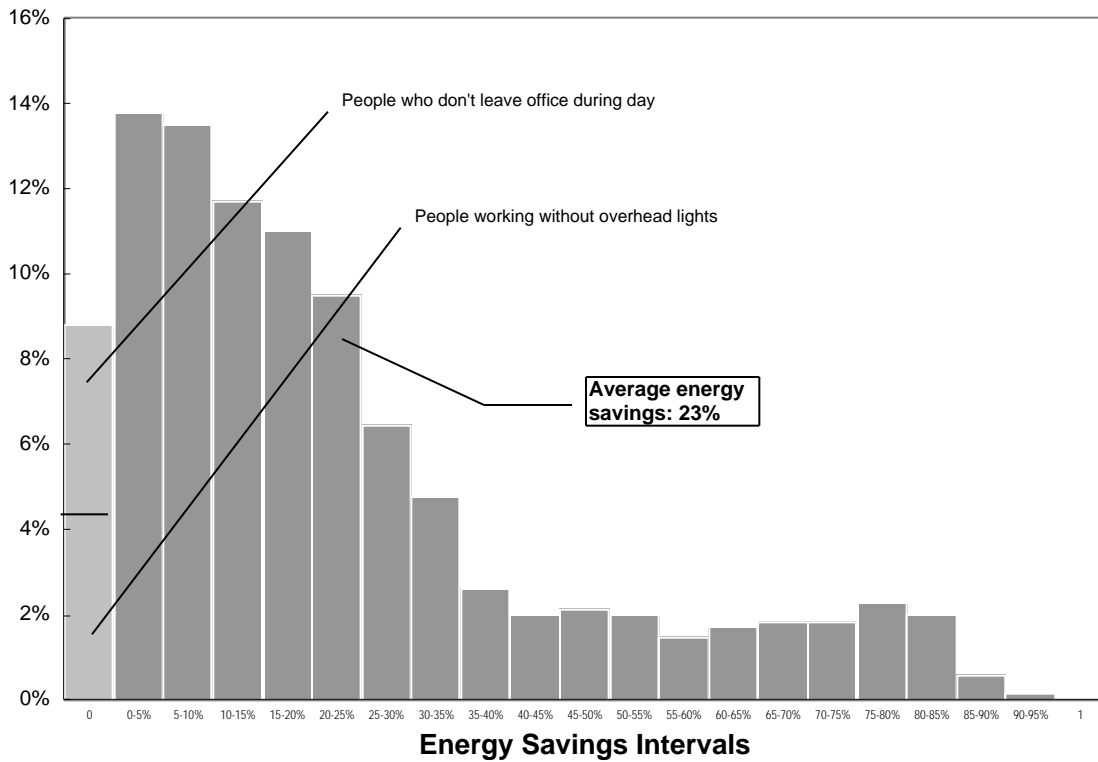
Figure 7. Daily energy savings from occupant sensors in 14 offices on the 5th floor for occupied days between June 1 and December 31, 1998. The energy savings by zone-day are binned into 5% intervals with a separate bin for days with exactly 0% energy savings.
