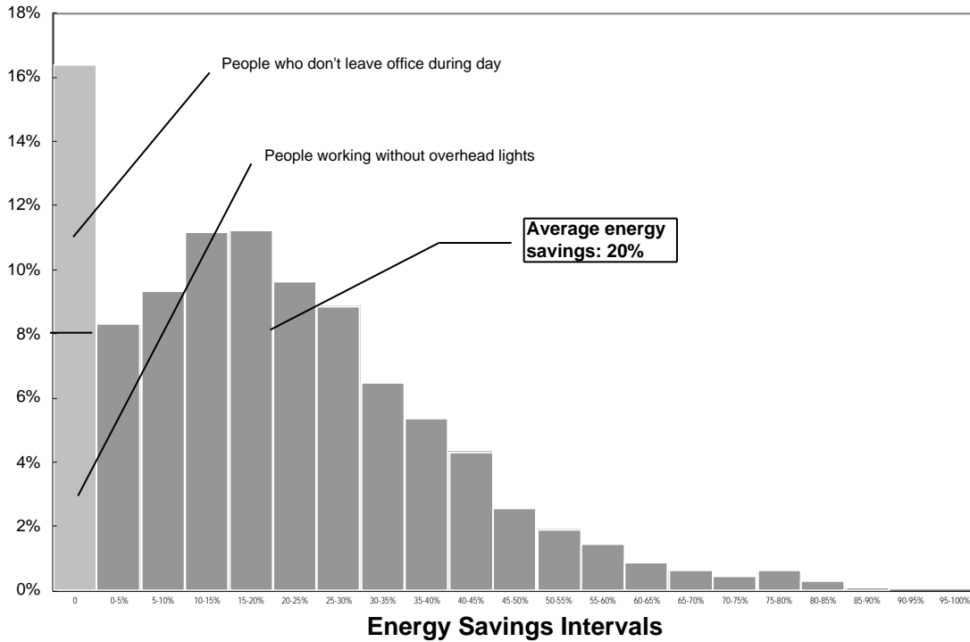
Figure 6. The energy savings from occupant sensors in 21 offices on the 3rd floor for occupied days between June 1 and December 31, 1998. The energy savings by zone-day are binned into 5% intervals with a separate
