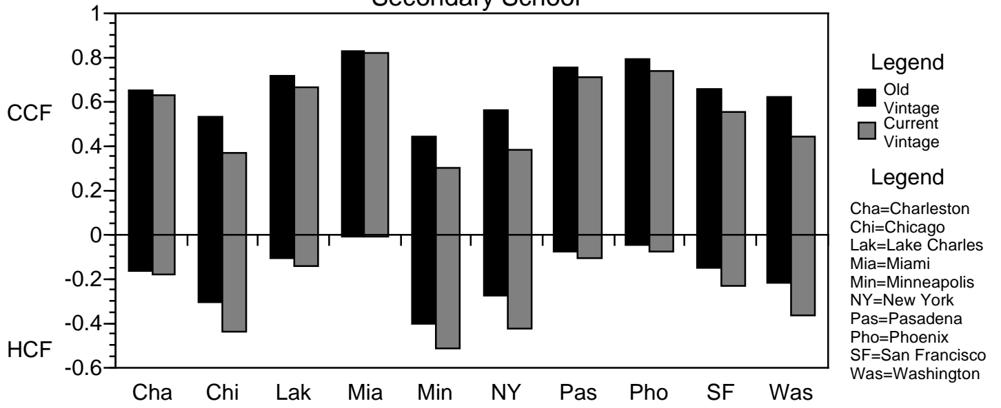
Figure 1. Heating and Cooling Coincidence Factors for Lighting (cont.) Secondary School
