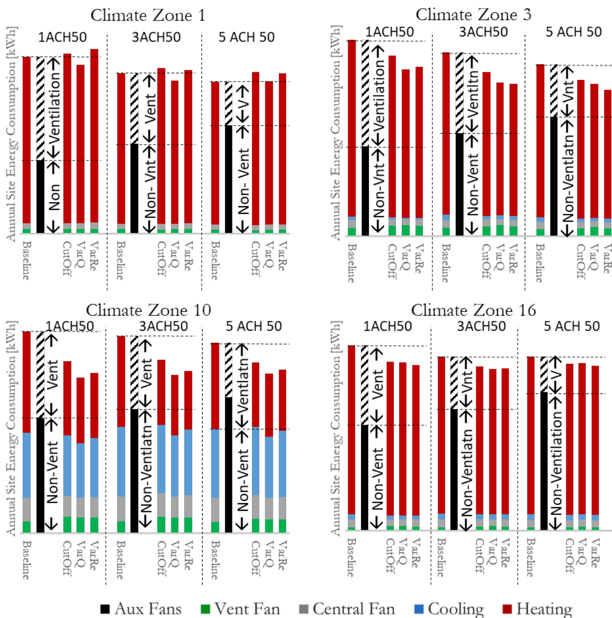
Figure 2 Annual consumption with best performing temperature-based smart ventilation control strategies. All results are for a single-story prototype home. Results are given for three different air-tightness levels as noted. Hatched regions denote energy associated with ventilation. Percentages refer to fraction of ventilation energy savings with best performing strategy.
