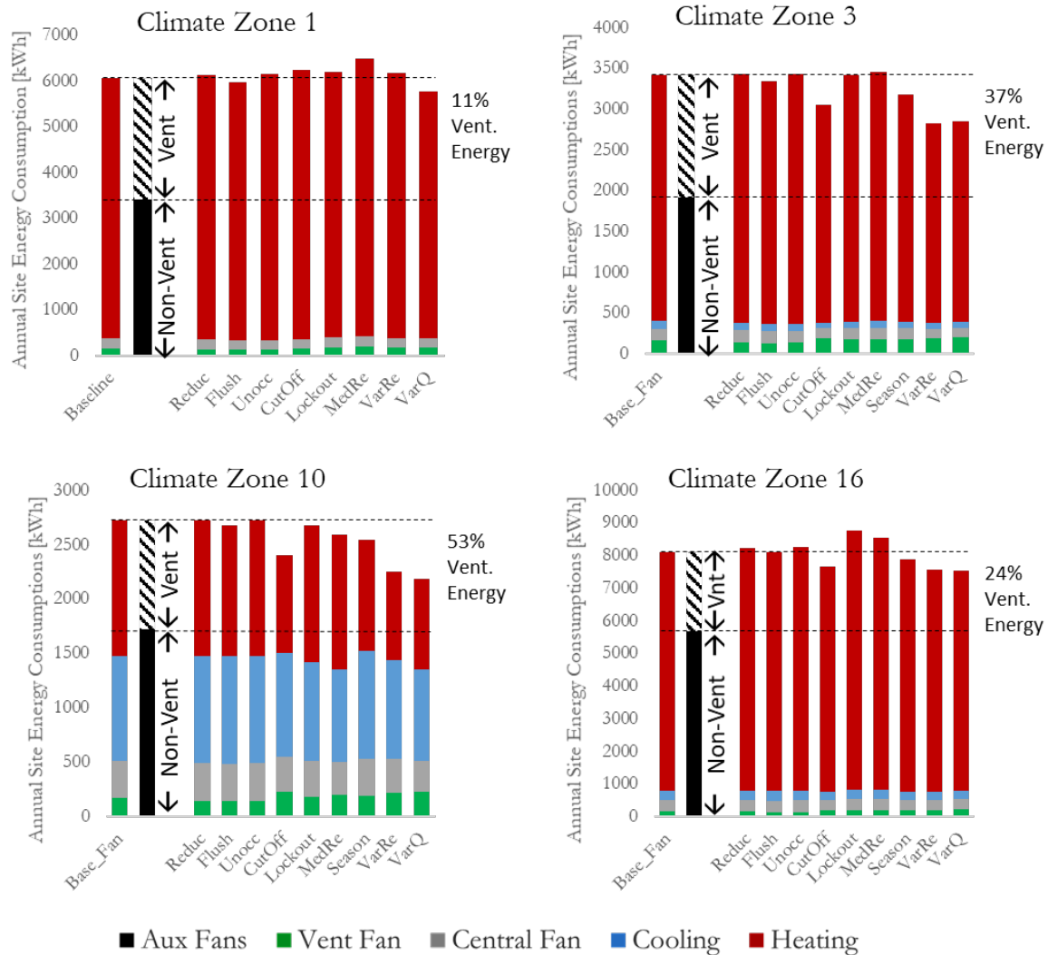
Figure 1 Modeled energy savings with each control strategy analyzed. Reported percentage of ventilation for each California climate zone refers to the percentage of energy associated with whole-house mechanical ventilation that is saved in the best-performing strategy. Diagonal hatches denote the portion of energy use associated with whole-house mechanical ventilation. Percentages refer to fraction of ventilation energy savings with best performing strategy.
