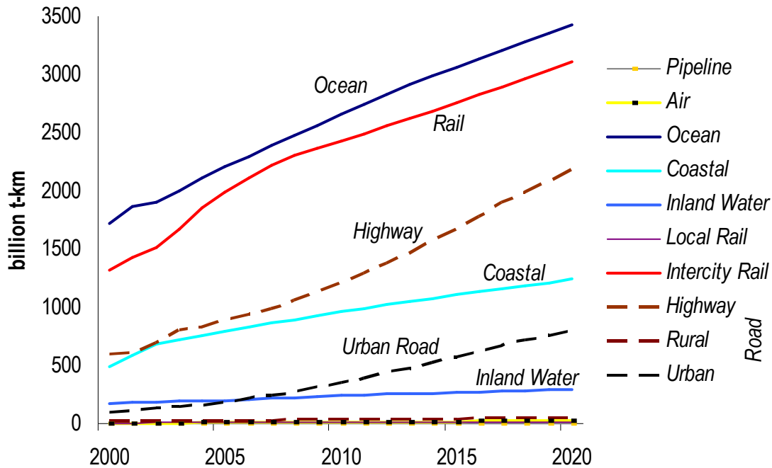
Figure 59 Freight Transport by Mode
