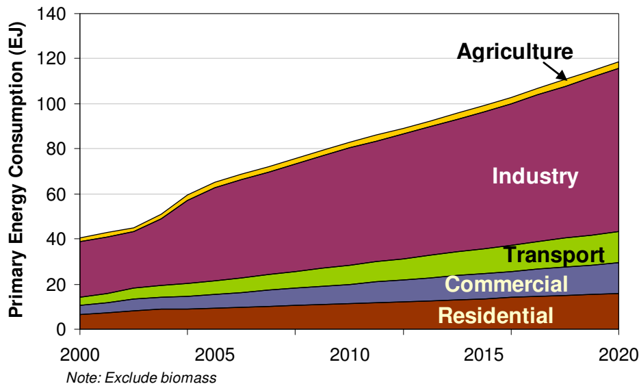
Figure 49 Primary energy consumption by sector
