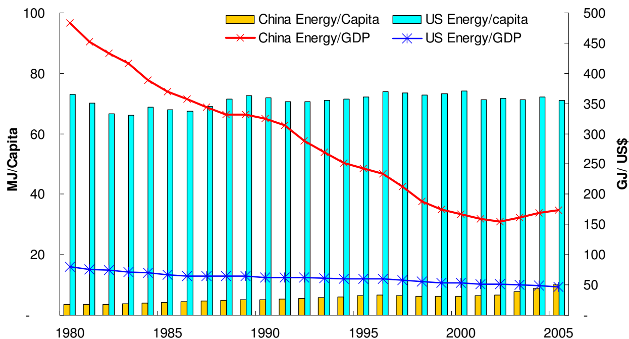
Figure 3 Energy Consumption per GDP and per Capita 4
