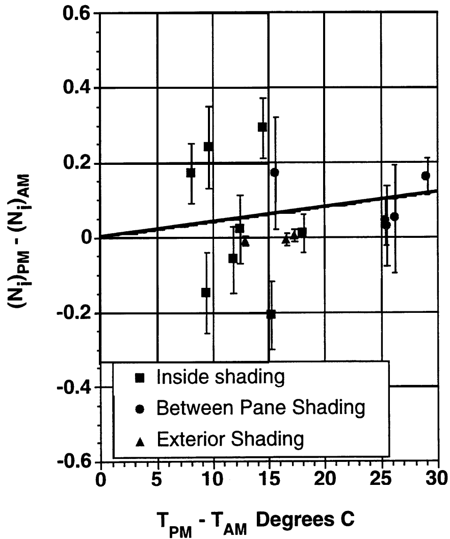
Figure 4. Changes in Inward- Flowing Fraction for a Shading layer in Direct Sunlight (PM) Compared with Darkness or Diffuse Daylight (AM), Verses Temperature Elevation Due to Sunlight. The solid curve is a fit to the between-pane shading data only.
