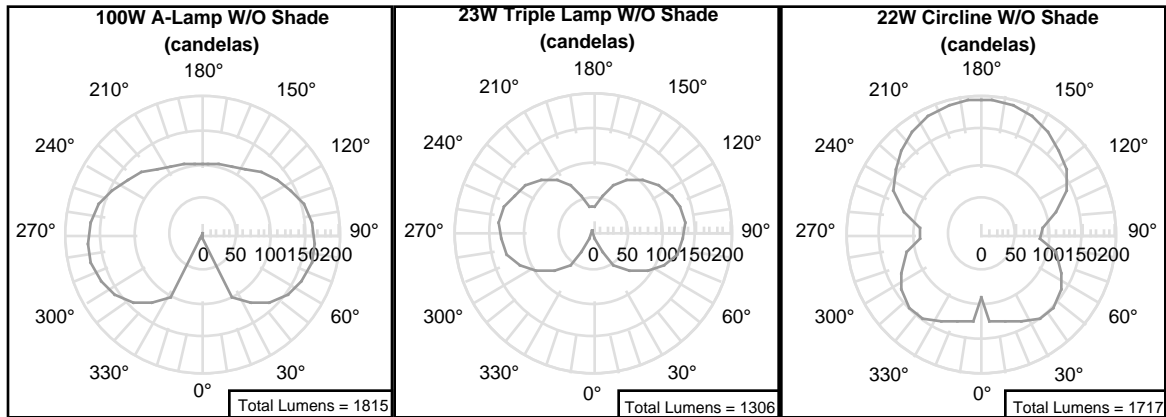
Figures 2a-c: Candela Plots of Table Lamps Operating without Shades.
