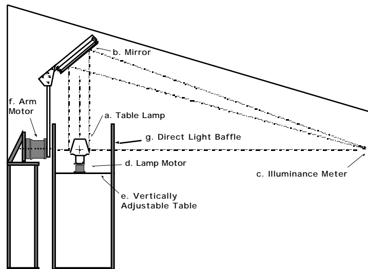
Figure 1: A Schematic of the Goniophotometer.
