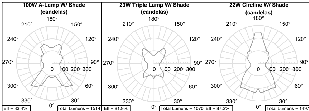
Figures 3a-c: Candela Plots of Table Lamps Operating with Shades.
