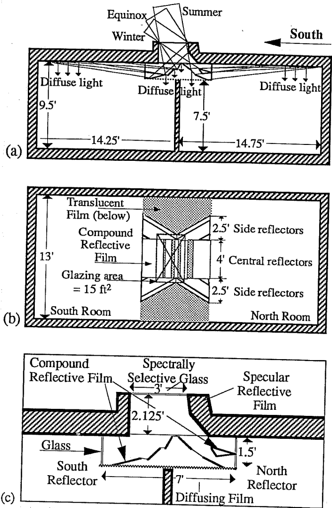
Figure 3. Skylight prototype: (a) Section along centerline of room, (b) View plan of skylight reflectors, and (c) Detail of reflectors.
