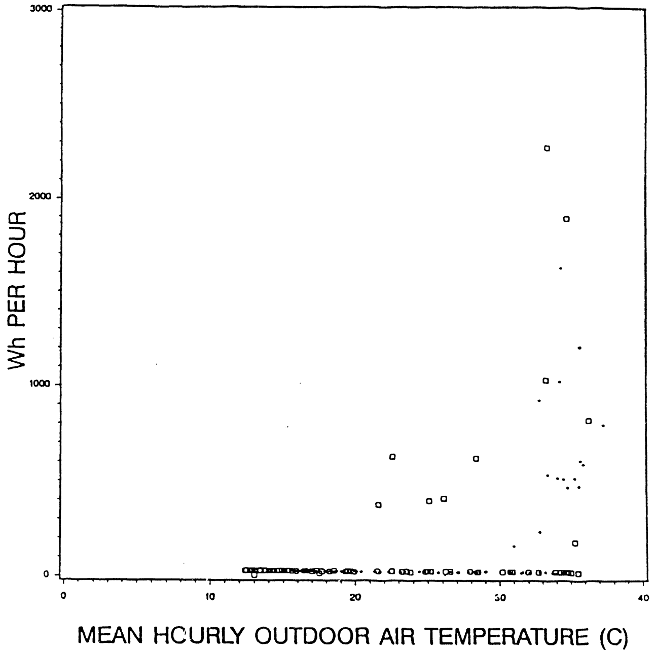
Figure V-4B. Site B: Hourly cooling electricity use (Wh/h) vs mean hourly outdoor air temperature (°C) for pre- and post-retrofit conditions at the test unit. The squares represent the pre-conditions (albedo = 0.08, brown), whereas the diamonds represent the post-conditions (albedo = 0.68, white). Monitoring period is from August 20 through September 2, 1991.
