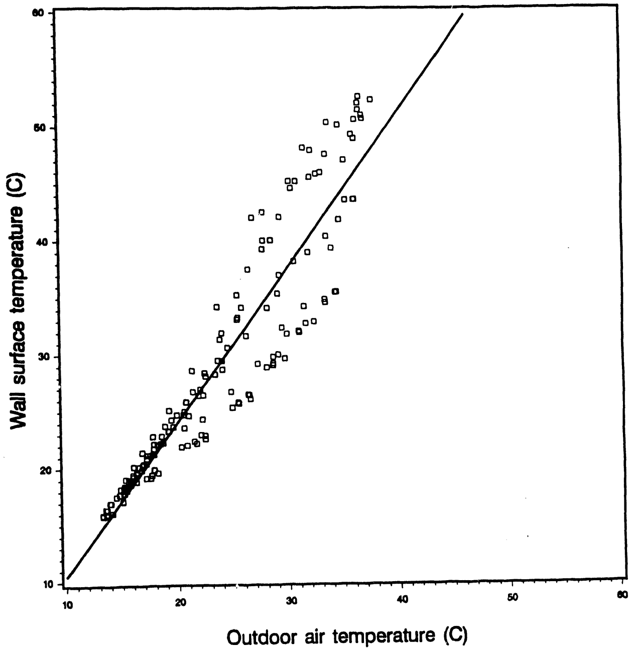
Figure V-6F. Site 6: West wall surface temperature ( ^{\circ}\text{C} ) vs outdoor air temperature ( ^{\circ}\text{C} ) for post-retrofit conditions. Solid line is regression fit to the data. Post-retrofit condition: two additional trees on west and one additional tree on south. Pre-retrofit monitoring period at this site was August 21 through September 22, and the post-retrofit period was September 25 through October 21, 1991.
