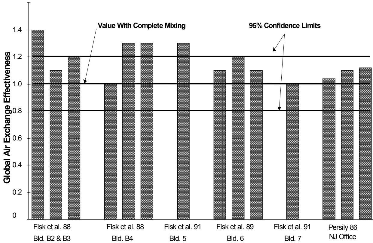
Figure 1. Results of field measurements of the global air exchange effectiveness. The 95% confidence limits are illustrated for a measurement with a value of 1.0.
