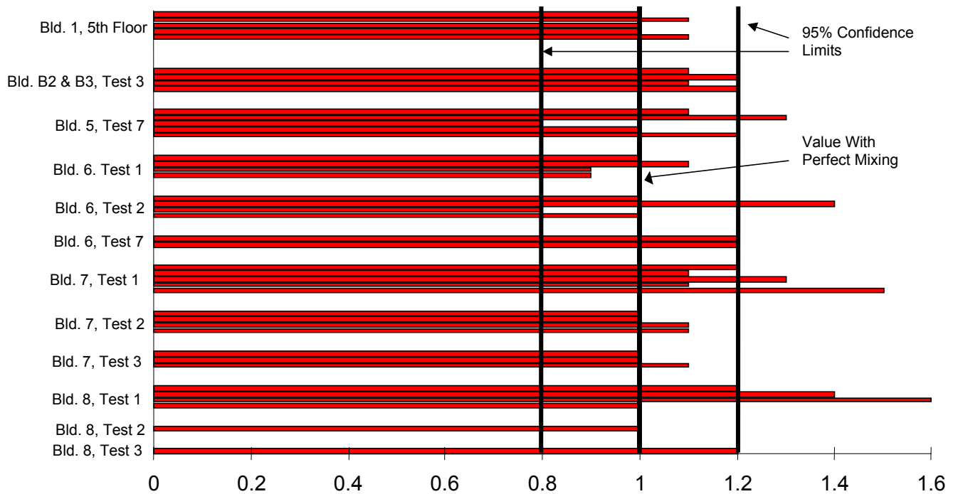
Figure 4. Results of field measurements of air diffusion effectiveness by the authors and colleagues ( Fisk et al. 1988, 1989, 1991). The 95% confidence limits are illustrated for a measurement with a value of 1.0.
