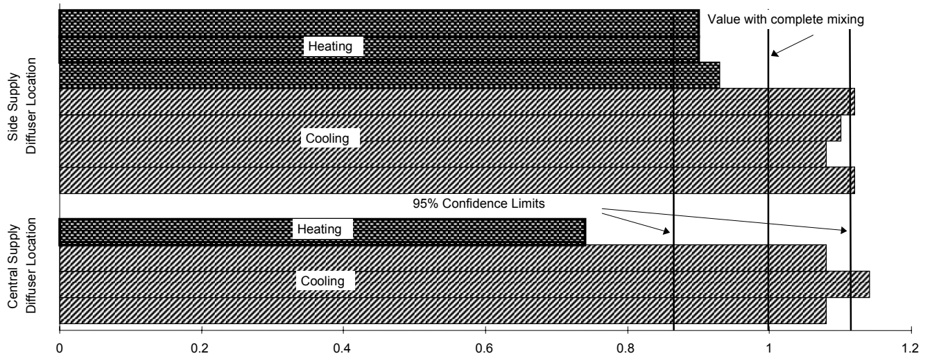
Figure 3. Results of measurement of breathing level air exchange effectiveness in the controlled environment chamber. The 95% confidence limits are illustrated for a measurement with a value of 1.0.
