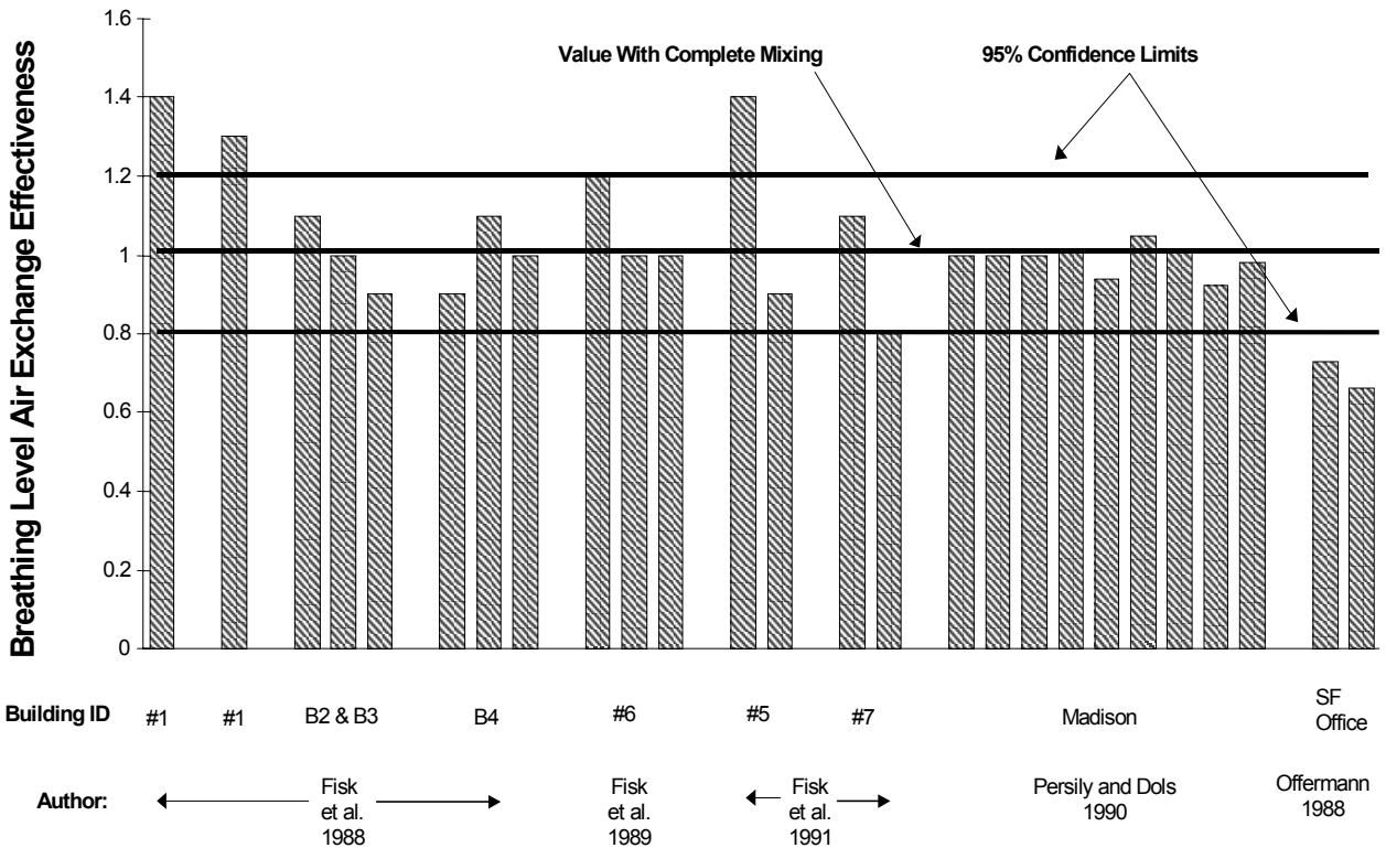
Figure 2. Results of field measurements of breathing level air exchange effectiveness. The 95% confidence limits are illustrated for a measurement with a value of 1.0.
