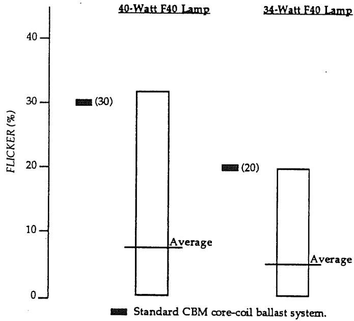
FIGURE 2.9 FLICKER FOR ELECTRONIC BALLASTS OPERATING F40 LAMPS
