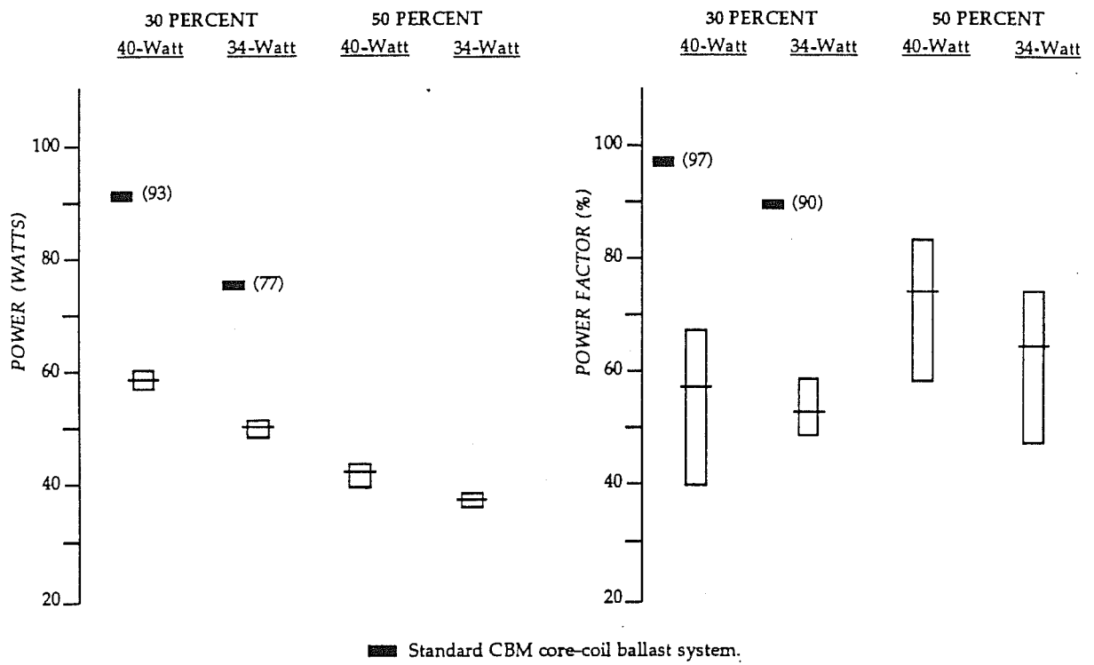
POWER AND POWER FACTOR FOR F40 LAMPS USING 30% AND 50% STATIC CONTROLLERS
