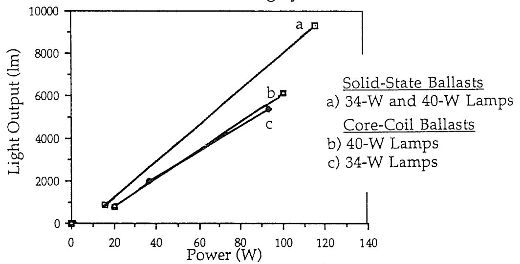
FIGURE 2.27 Light Output vs Power Input For The Dimming Systems
