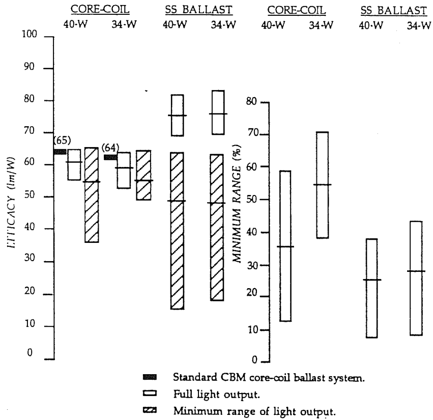
FIGURE 2.22 SYSTEM EFFICACY AND MINIMUM DIMMING RANGE OF DYNAMIC CONTROLS
