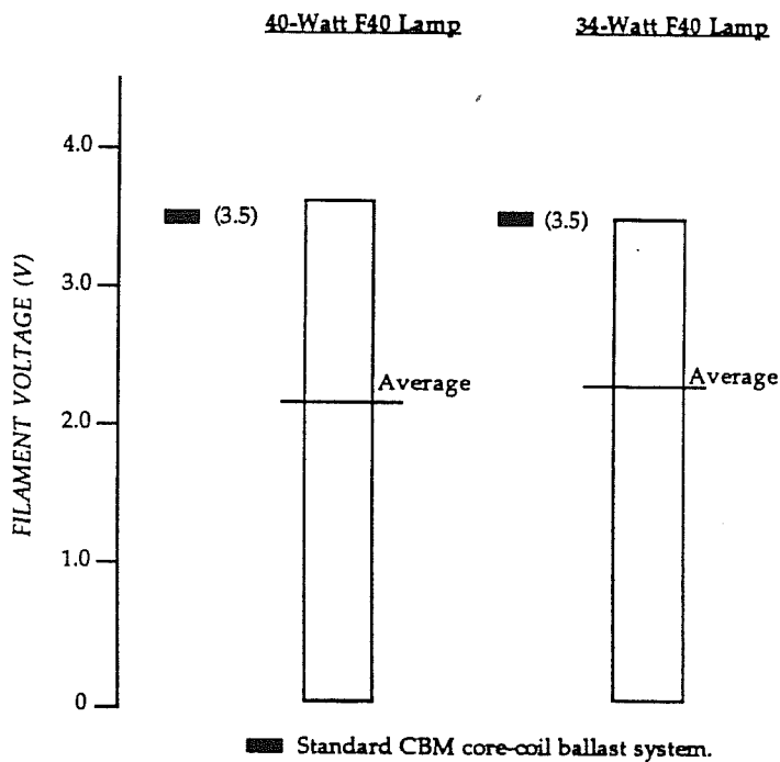
FIGURE 2.5 FILAMENT VOLTAGE FOR ELECTRONIC BALLASTS OPERATING F40 LAMPS
