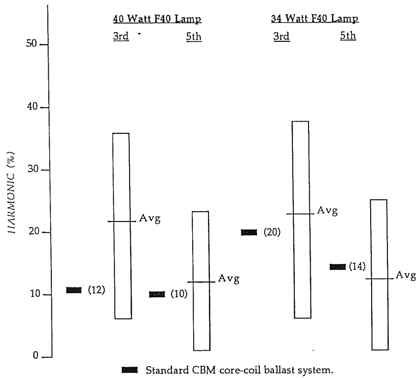
FIGURE 2.3 THIRD AND FIFTH HARMONIC FOR ELECTRONIC BALLASTS OPERATING F40 LAMPS
