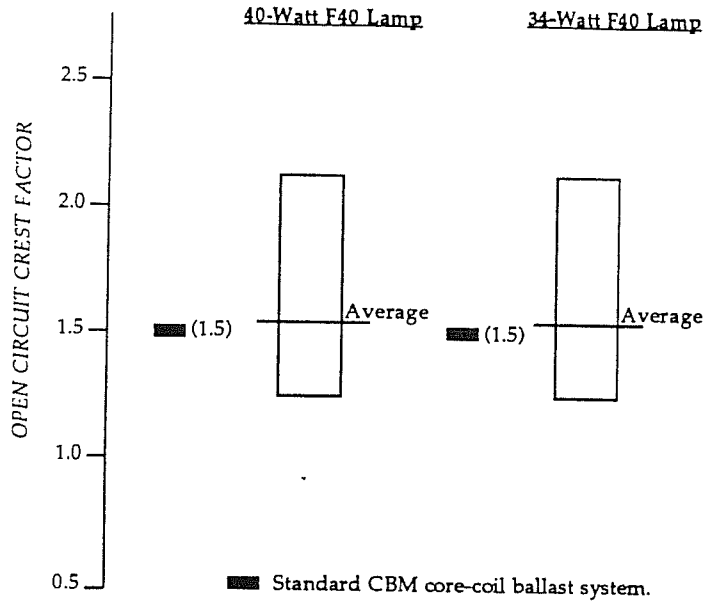
FIGURE 2.8 OPEN CIRCUIT CREST FACTOR FOR ELECTRONIC BALLASTS OPERATING F40 LAMPS
