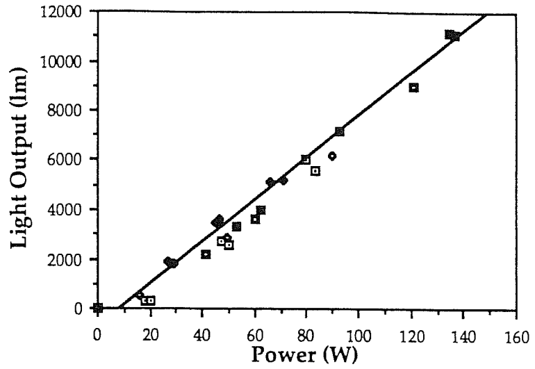
FIGURE 2.23 Light Output for 40W Lamps With Solid-State Ballasts
