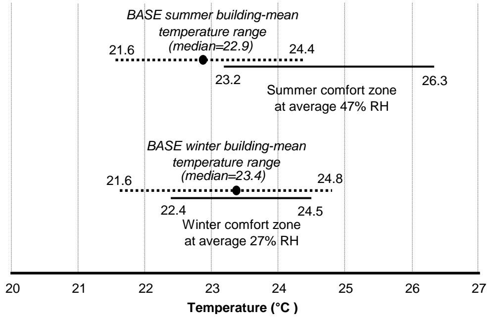
Figure 1. Observed indoor temperatures in BASE buildings relative to recommended thermal comfort guidelines (ASHRAE, 2005b), by season
