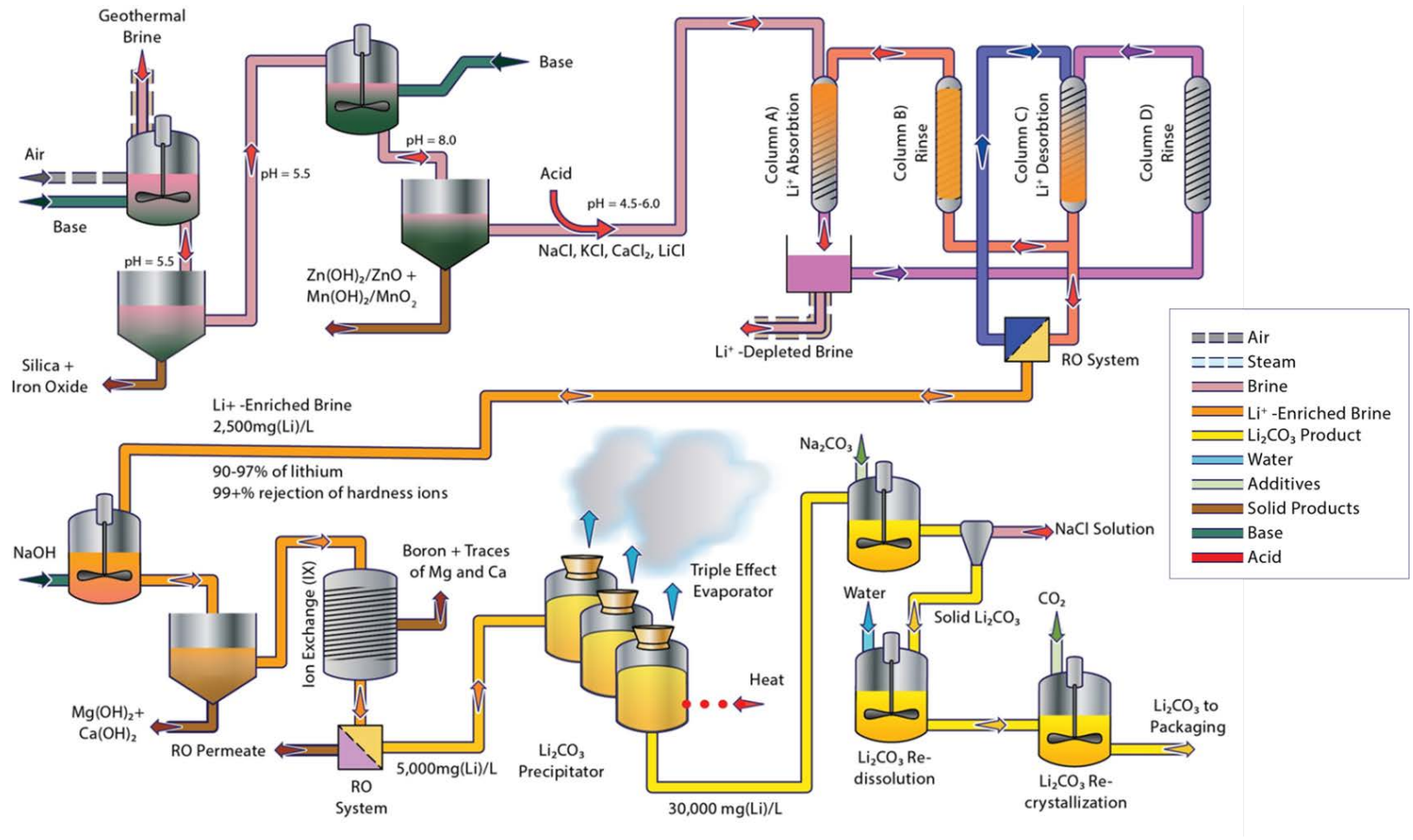
Figure 9.9. Conceptual process for the extraction and refining of lithium from geothermal brines from the SS-GR.
