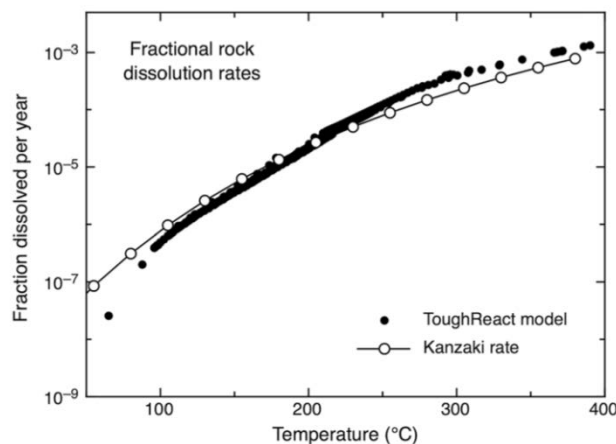
Figure 6.8. Comparison of effective dissolution rates calculated using TOUGHREACT for Mid-ocean Ridge basalts to experimental rates based on oxygen exchange (DePaolo et al., 2022).
