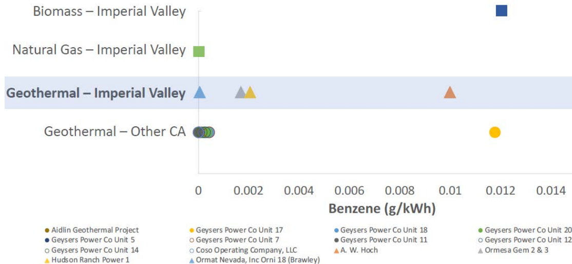
Figure 8.10. Comparison of benzene emission rates from geothermal energy production in California and Imperial Valley to biomass and natural gas facilities reporting emissions in the Salton Sea Air Basin.
