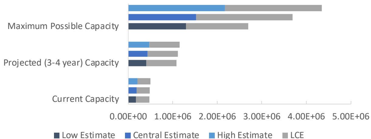
Figure 8.17. Estimated CO 2 emissions from geothermal expansion scenarios using low/medium/high emission rates from Table 8.3 and estimated emissions for the associated lithium production potential for each scenario.
