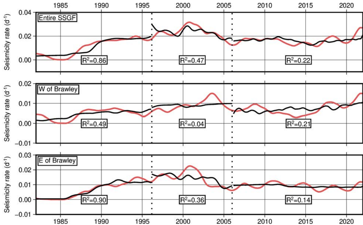
Figure 10.2. Background seismicity rate for a) the entire Focus Region, b) the region W of the Brawley Fault, and c) the region E of the Brawley Fault. Estimated from the Augmented Hauksson et al. (2012) catalog using the NND de-clustered catalog. Solid black curves show the piecewise-linear hindcast model. Dotted black lines represent discontinuities in the hindcast model. R^2 values quantify the correlation between the observed seismicity rate and hindcast model for each time period.
