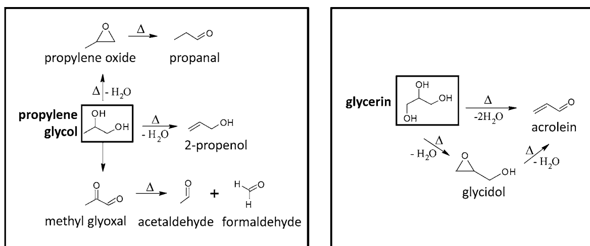
Figure 6. Postulated pathways and byproducts formed during thermal dehydration of propylene glycol and glycerin.
