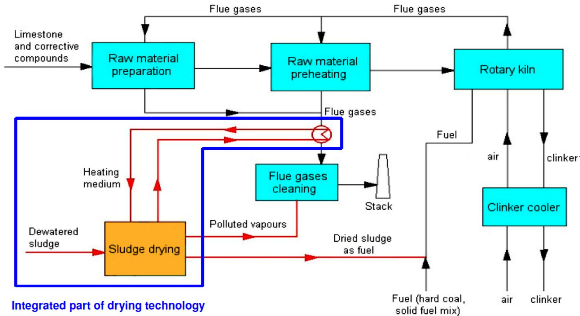
Figure 23. Using cement plant's flue gas heat for sludge drying (Stehlík et al., no date)
