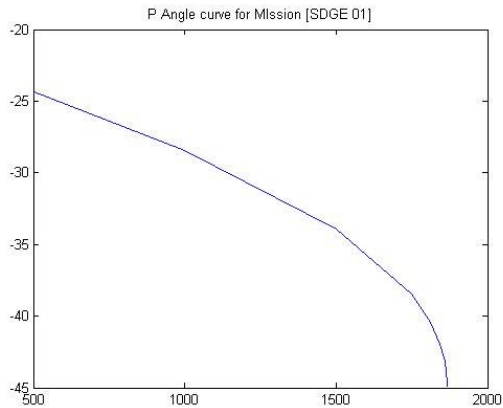
Figure 17 P Angle Curve for Mission with Stress Pattern III Showing Collapse Source: CERTS
