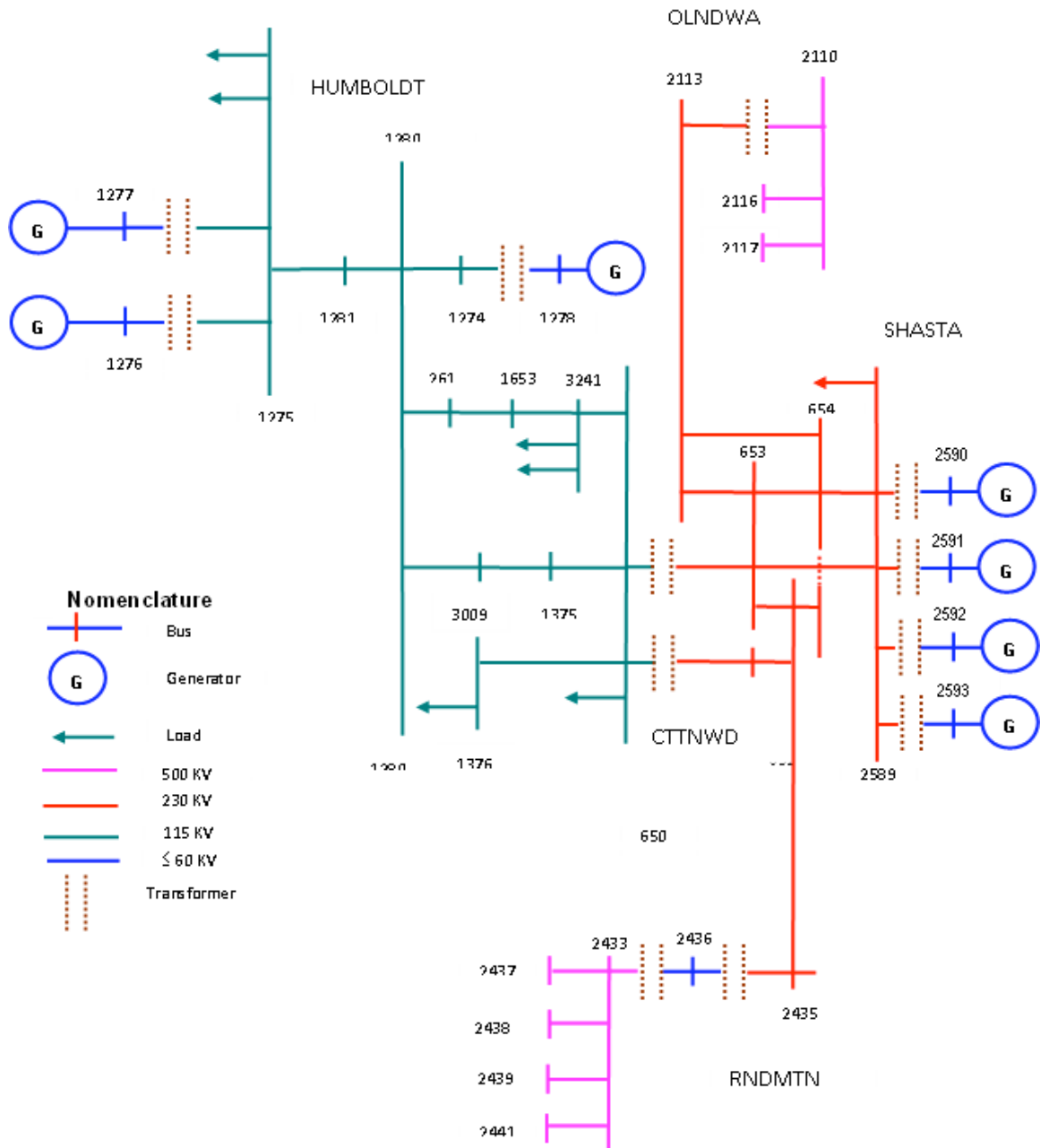
Figure 21 One Lines for the HUMBOLDT CTTNWD SHASTA Area Source: CERTS
