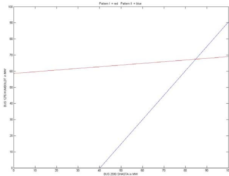
Figure 22 RTVSA Output: Hyperplane Slices at Humboldt 1276 and Shasta 2590 Source: CERTS
