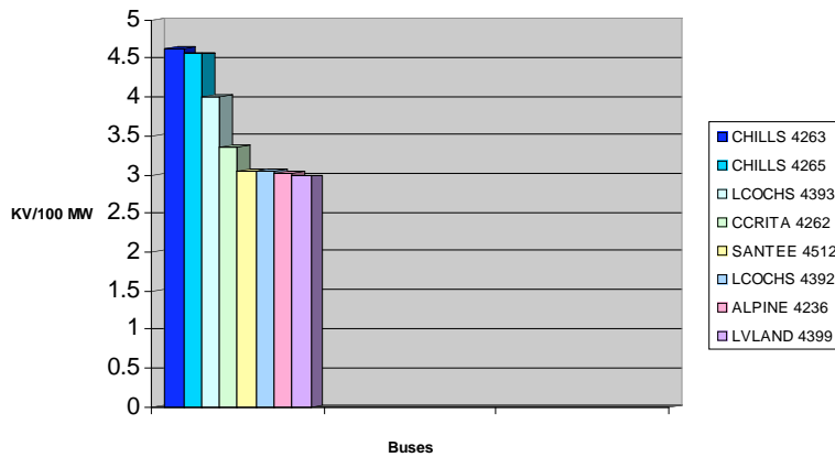
Figure 13 Top Eight Voltage Collapse Participation Factors for Stressing Pattern I Source: CERTS
