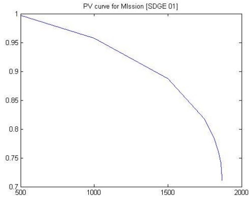
Figure 16 PV Curve for Mission with Stress Pattern III Showing Collapse Source: CERTS
