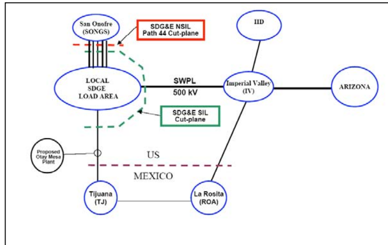
Figure 5 Major Import Paths in the SDGE System Source: CERTS
