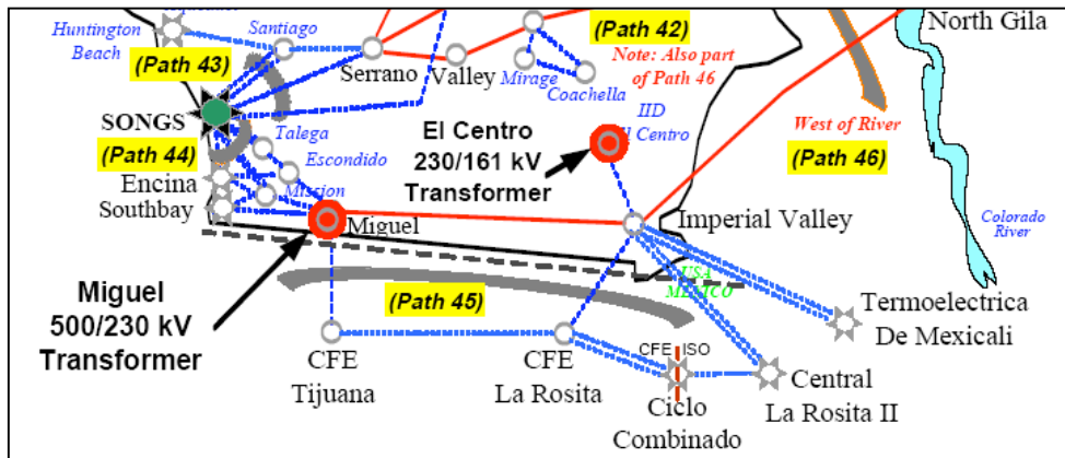
Figure 7 Location of Songs and South Bay in the CA EHV Transmission Network Source: CERTS
