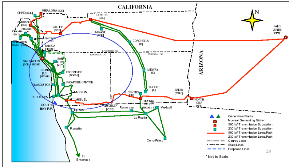
Figure 6 Map Showing the Two Arms of the SWPL Corridor in Relation to SDGE Source: CERTS
