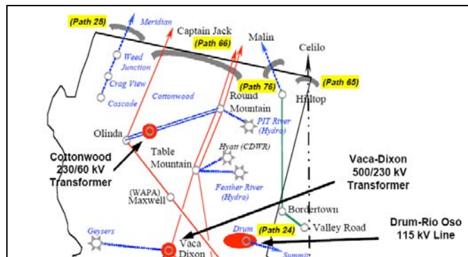
Figure 20 Location of Cottonwood in the CA EHV Transmission Network Source: CERTS
