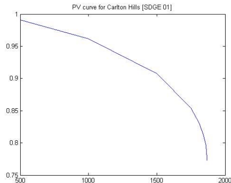
Figure 15 PV Curve for Carlton Hills with Stress Pattern III Showing Collapse Source: CERTS
