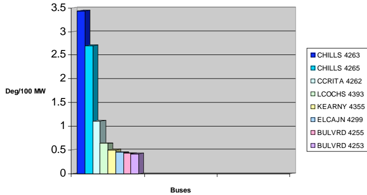
Figure 14 Top Eight Angle Collapse Participation Factors for Stressing Pattern I Source: CERTS
