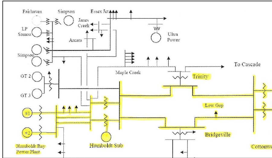
Figure 19 Humboldt Area Source: CERTS
