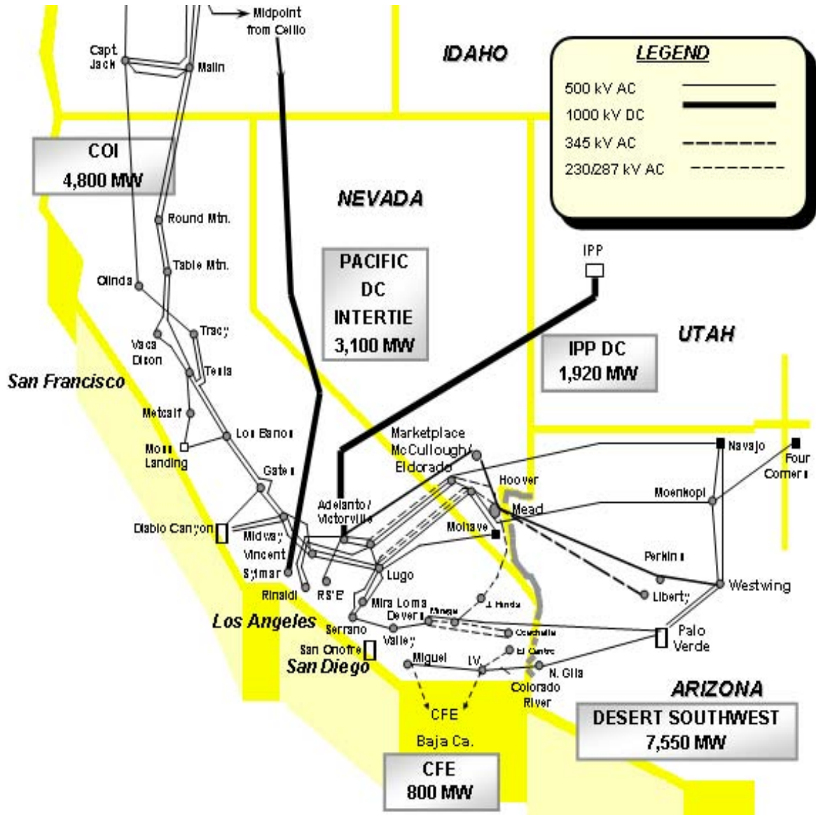
Figure 2 – California’s 18,170 MW of EHV Transmission Interconnections
