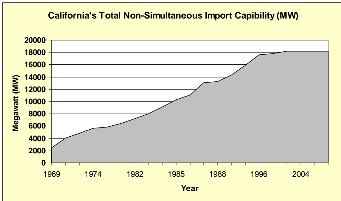
Figure 1 – California Non-Simultaneous Import Capability
