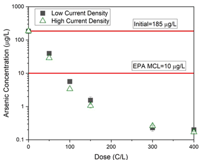
Fig. 2. Arsenic concentration (µg/L) in the filtered samples at various charge dose (Batches number 3-5). Note vertical scale is logarithmic. All data taken in high conductivity period. Data at 0, 50, 100 C/L are duplicate measurements and everything else is triplicate. Standard deviations are indicated by vertical error bars.
