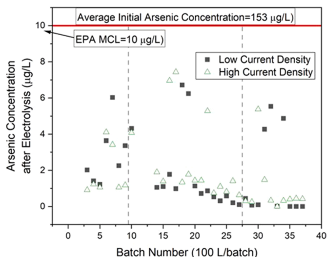
Fig. 3. Arsenic concentration (µg/L) after electrolysis during field trial at 150 C/L (Batch number 3-37). Note linear vertical scale. Batches 11-13 not included in figure as the samples were lost from improper filtration (see text). Two dotted lines demarcate conductivity periods (1-9 and, 28-37 are “high conductivity”, and 10-27 is “low conductivity”). The measurement error on each sample point was less than 5% and therefore not shown in the graph for brevity.
