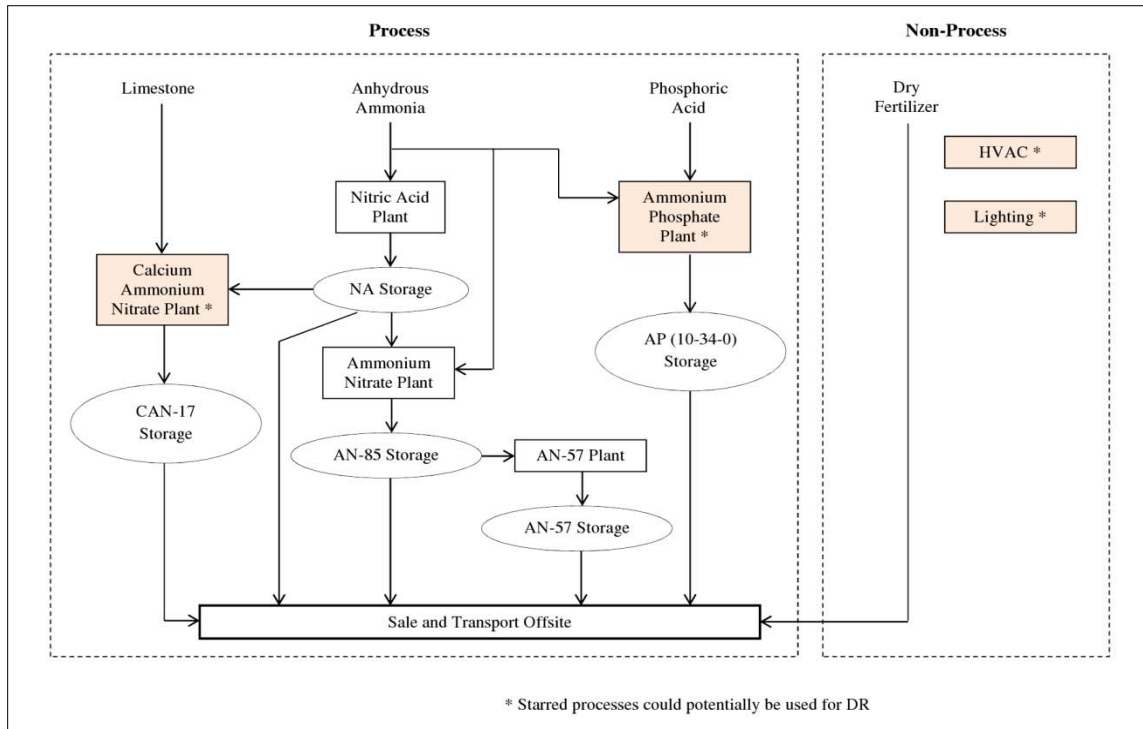
Figure 6: A process flow diagram of J.R. Simplot's Helm facility.
