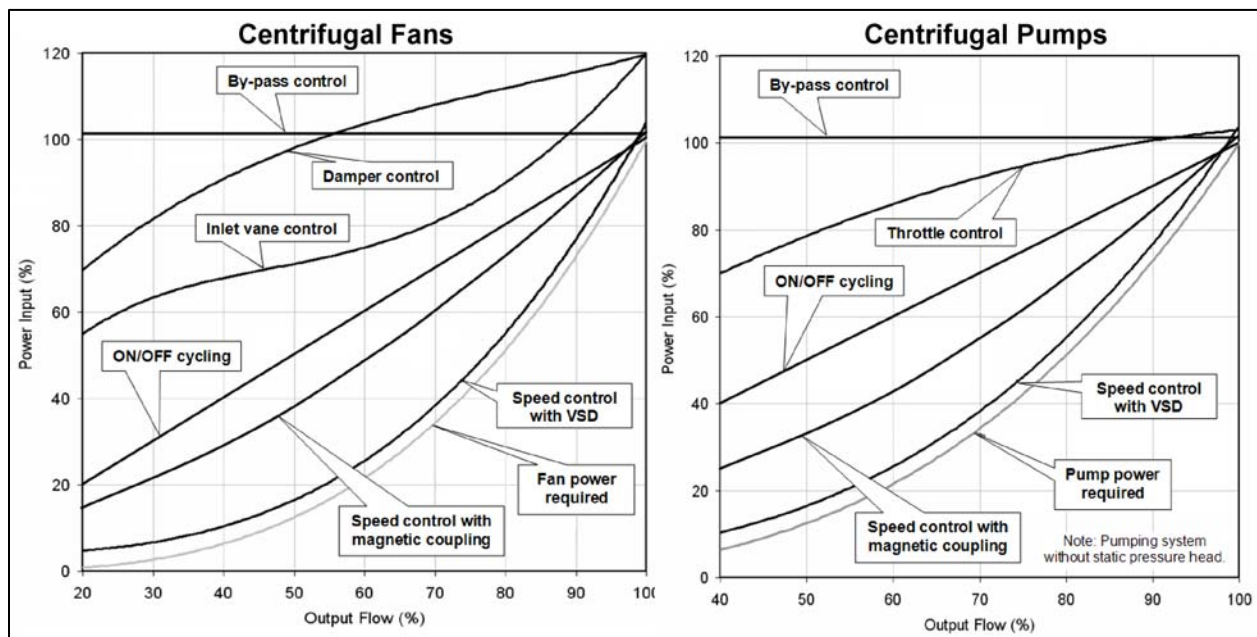
Figure 7: Comparison of a partial-flow power consumption in pumps and fans with various methods of flow control. Source: Ferreira 2009
