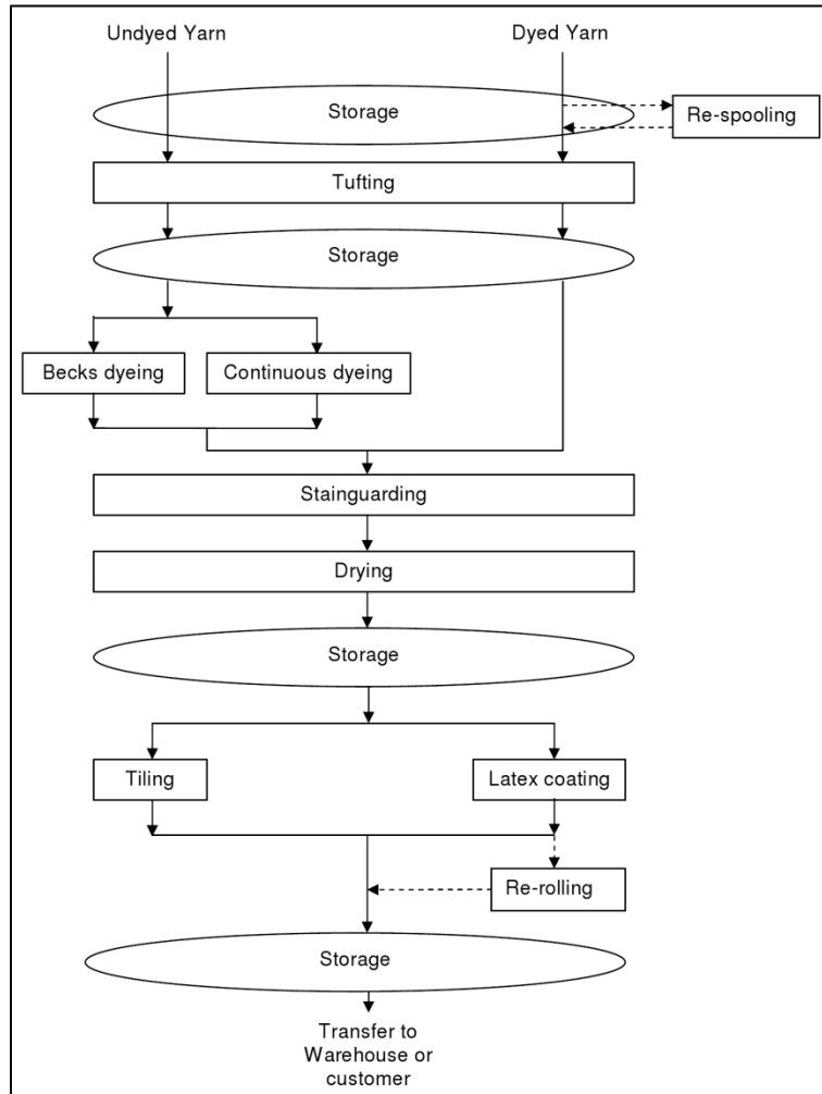
Figure 4: Process flow diagram for Bentley Prince Street’s manufacturing facility.
