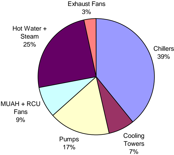
Figure 1. Benchmarked HVAC energy usages in a semiconductor cleanroom facility
