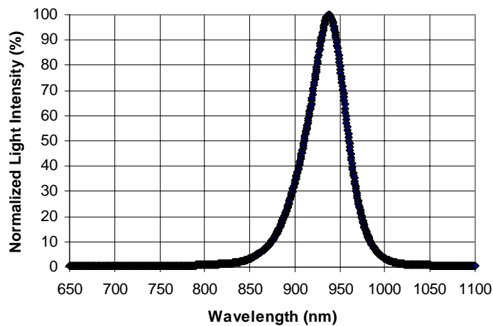
Figure 6. Spectrum of infrared light-emitting diode.
