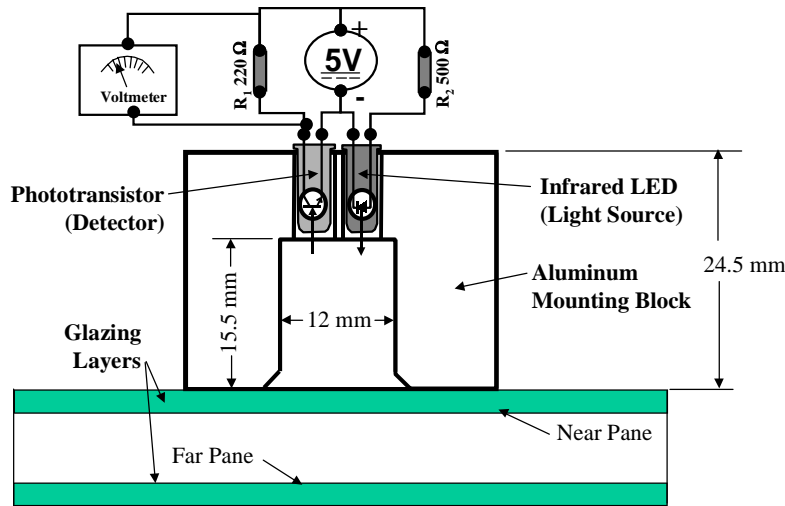
Figure 7. Test setup for IR-LED/phototransistor pair.
