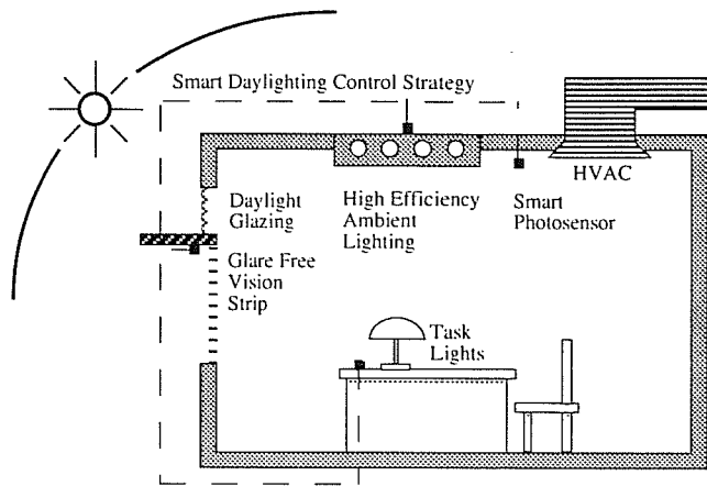
Figure 5. Core Daylighting Systems Concept.
