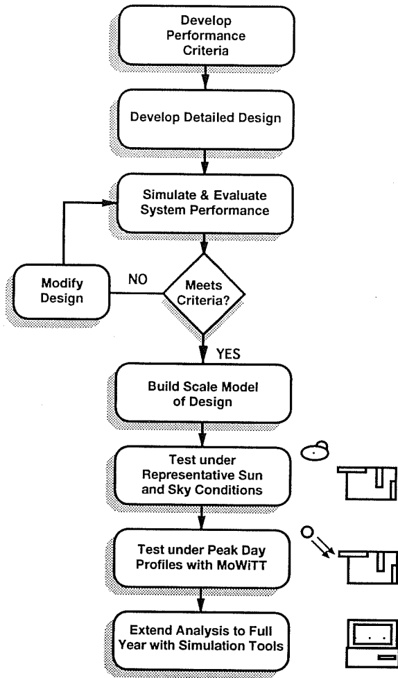
Figure 6. An iterative development sequence was used to design the integrated envelope and lighting prototypes. Initial designs were evaluated using quick analysis methods. Refined designs were then evaluated using more extensive laboratory and field test measurements as well as comprehensive simulation tools.
